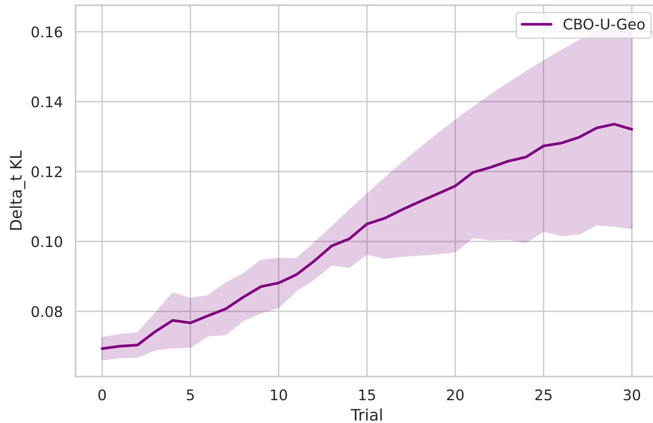
Erdos20 (nonlinear)
