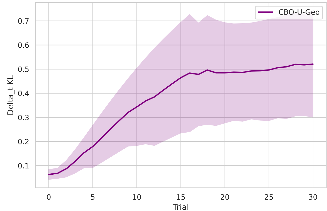
Erdos100 (nonlinear)
