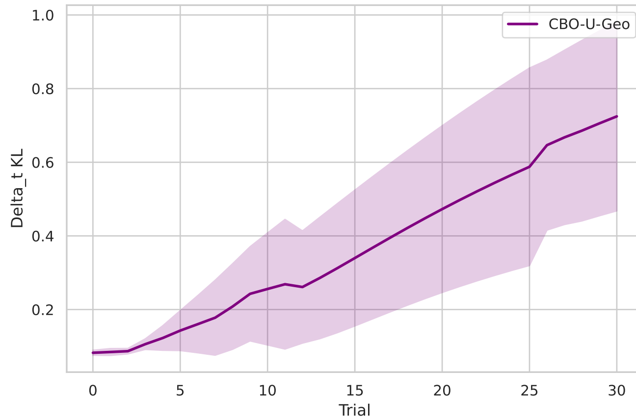
Erdos50 (nonlinear)
