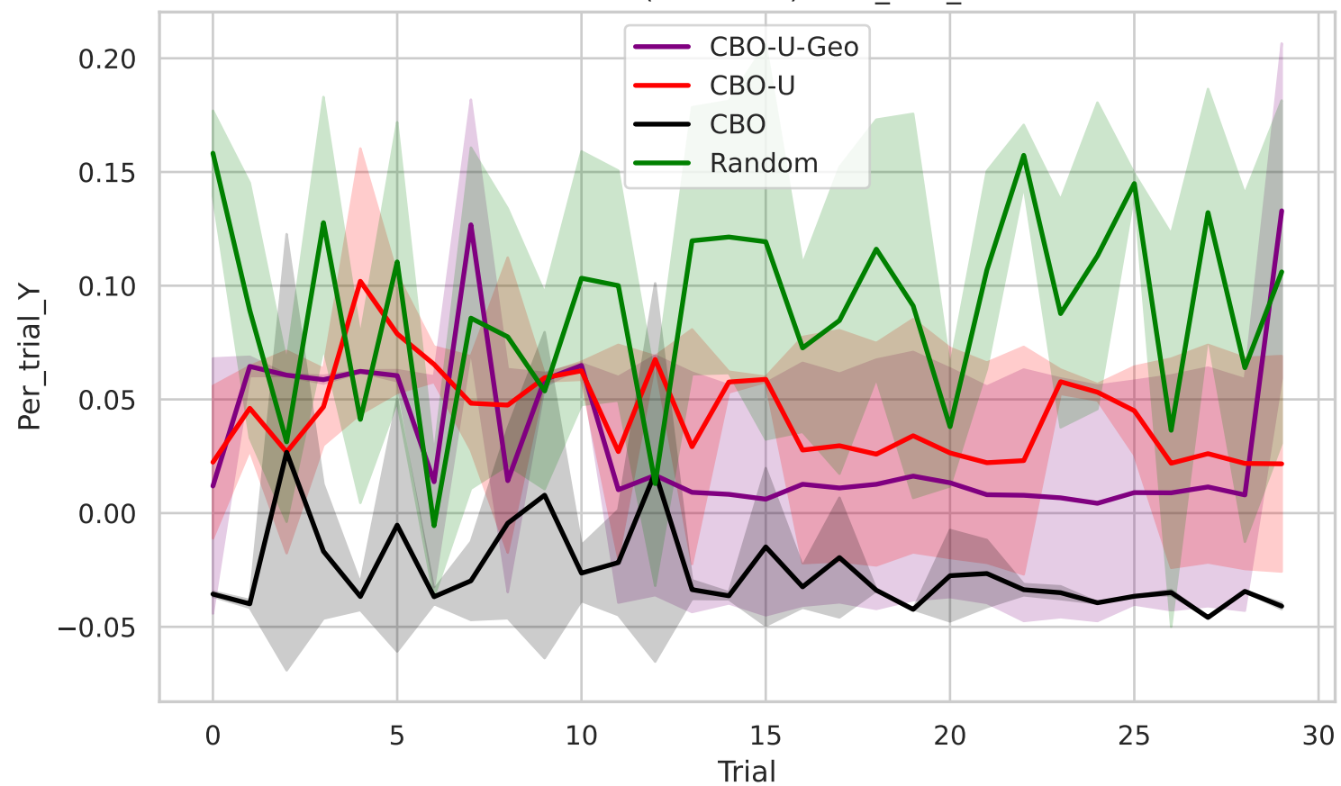
Erdos20 (nonlinear) - Per_trial_Y
