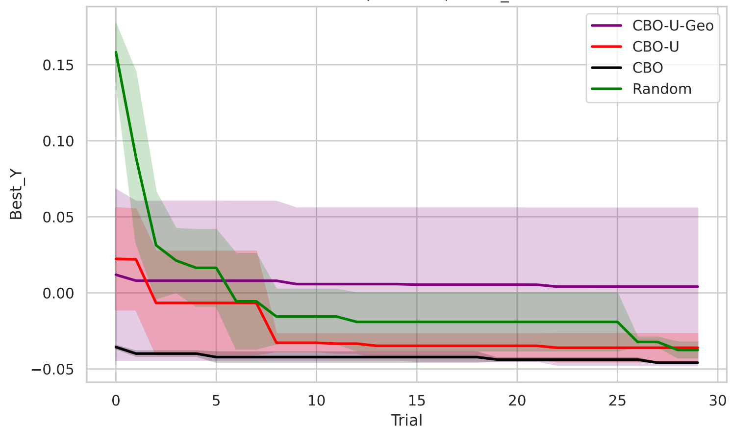
Erdos20 (nonlinear) - Best_Y
