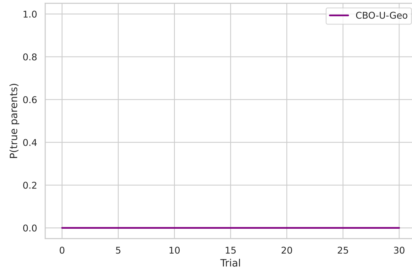
Erdos100 (nonlinear)
