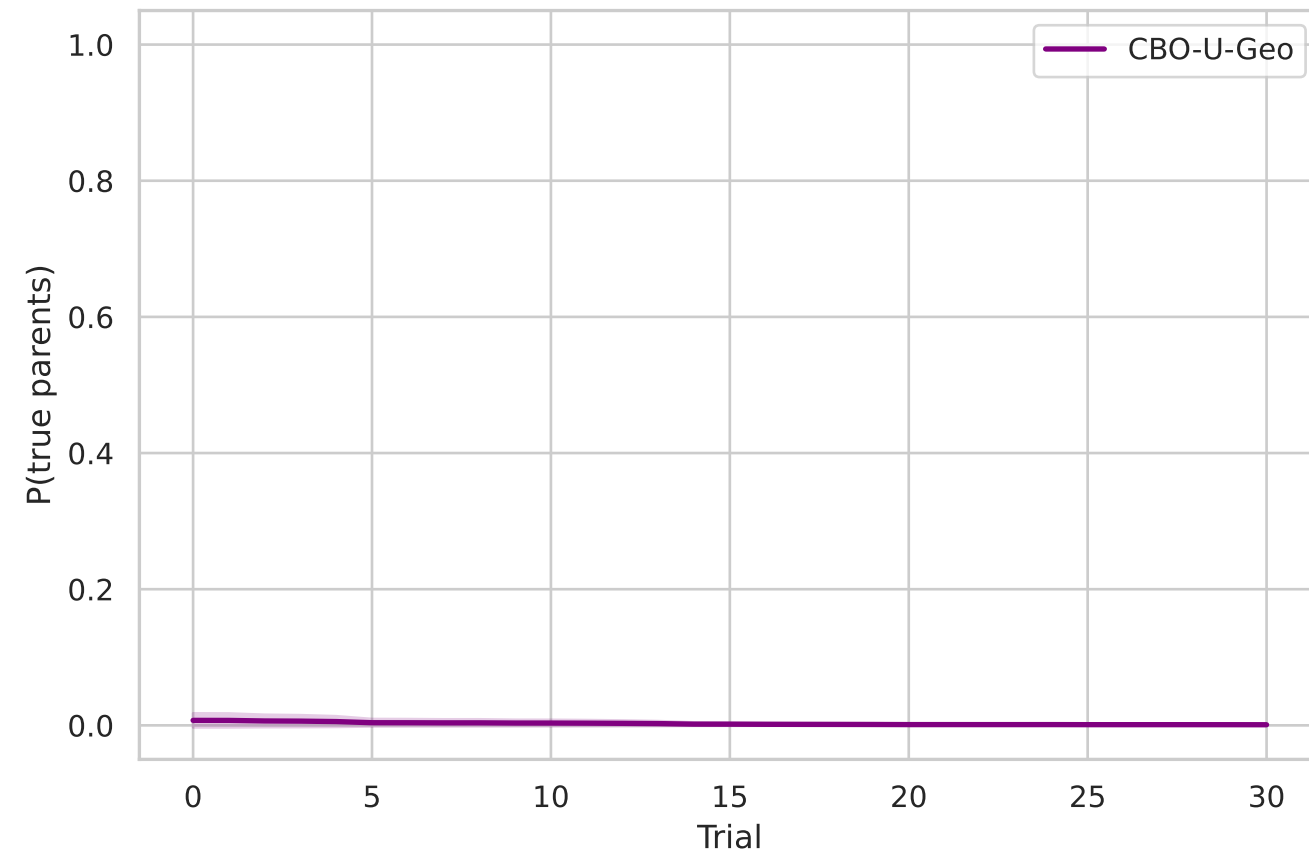
Erdos50 (nonlinear)
