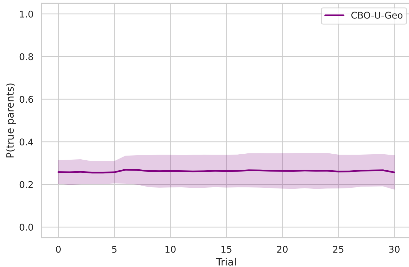
Erdos20 (nonlinear)
