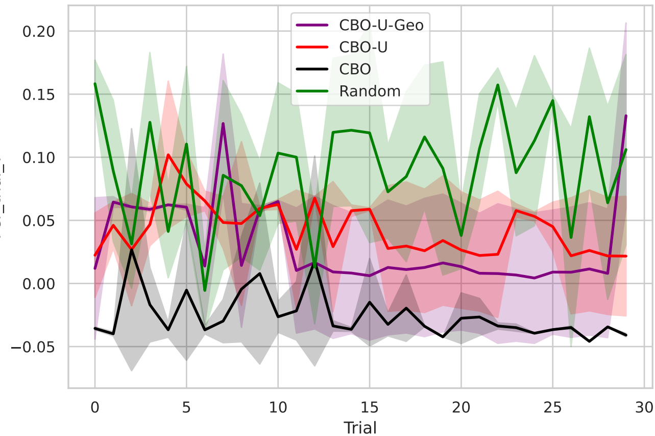
Erdos20 (nonlinear)
