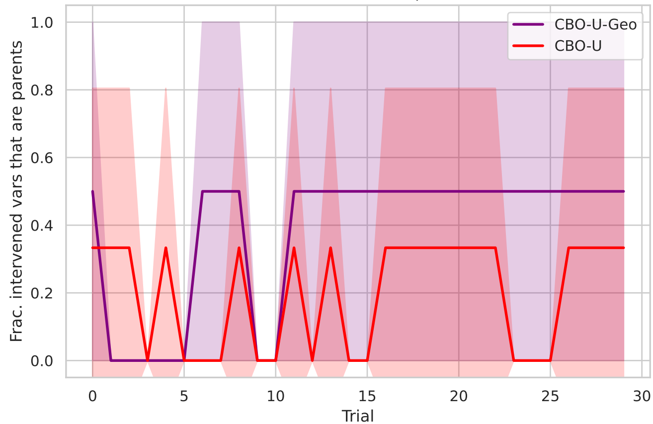
Erdos20 (nonlinear) - true parents ['4']
