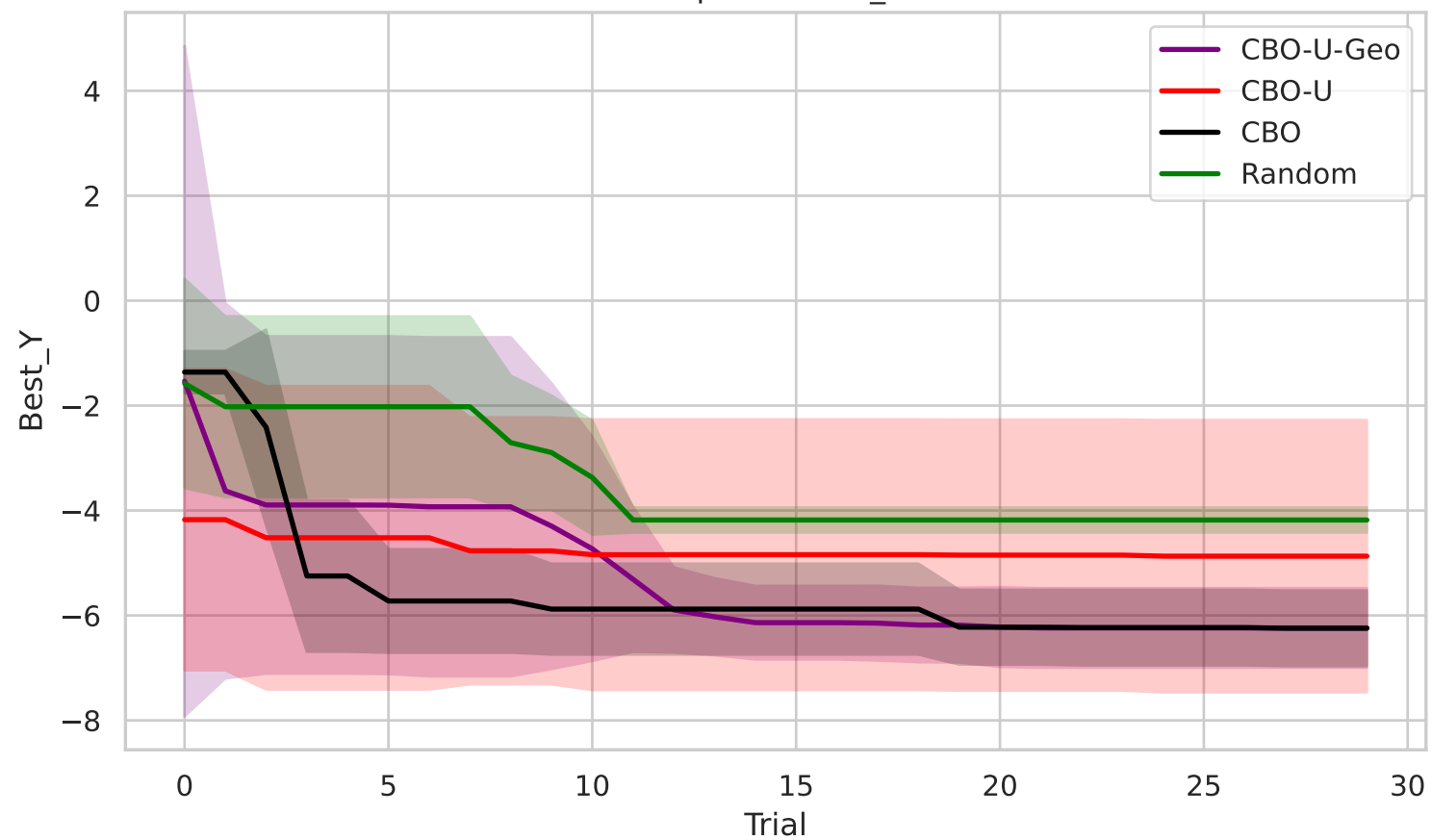
Gwps60 - Best_Y
