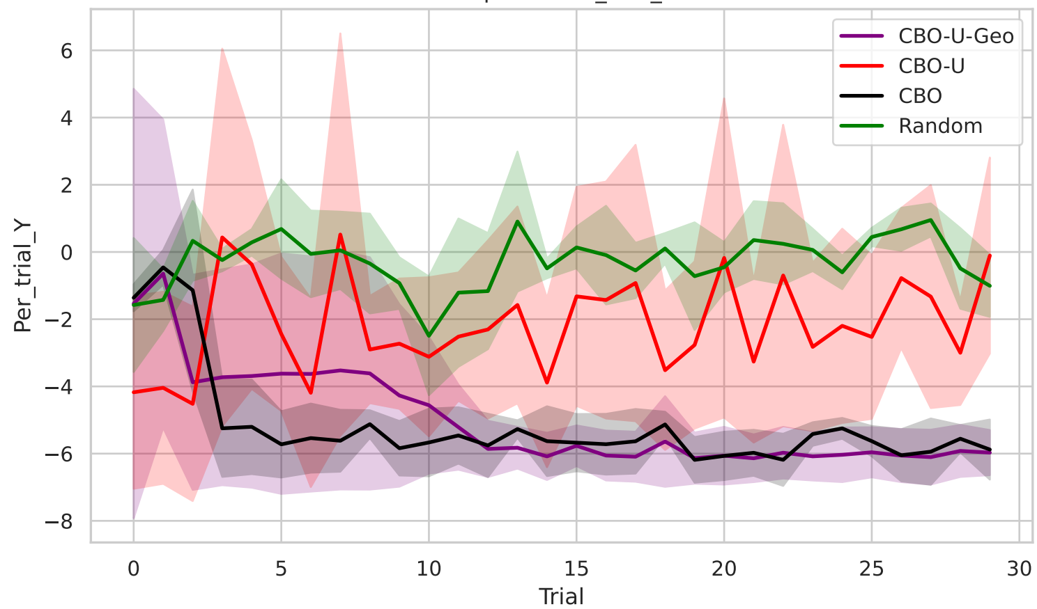
Gwps60 - Per_trial_Y
