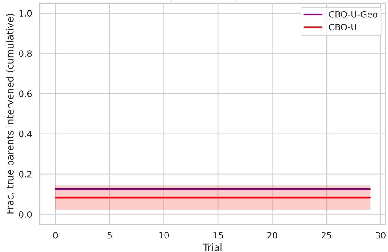
Gwps60 - 8 true parents
