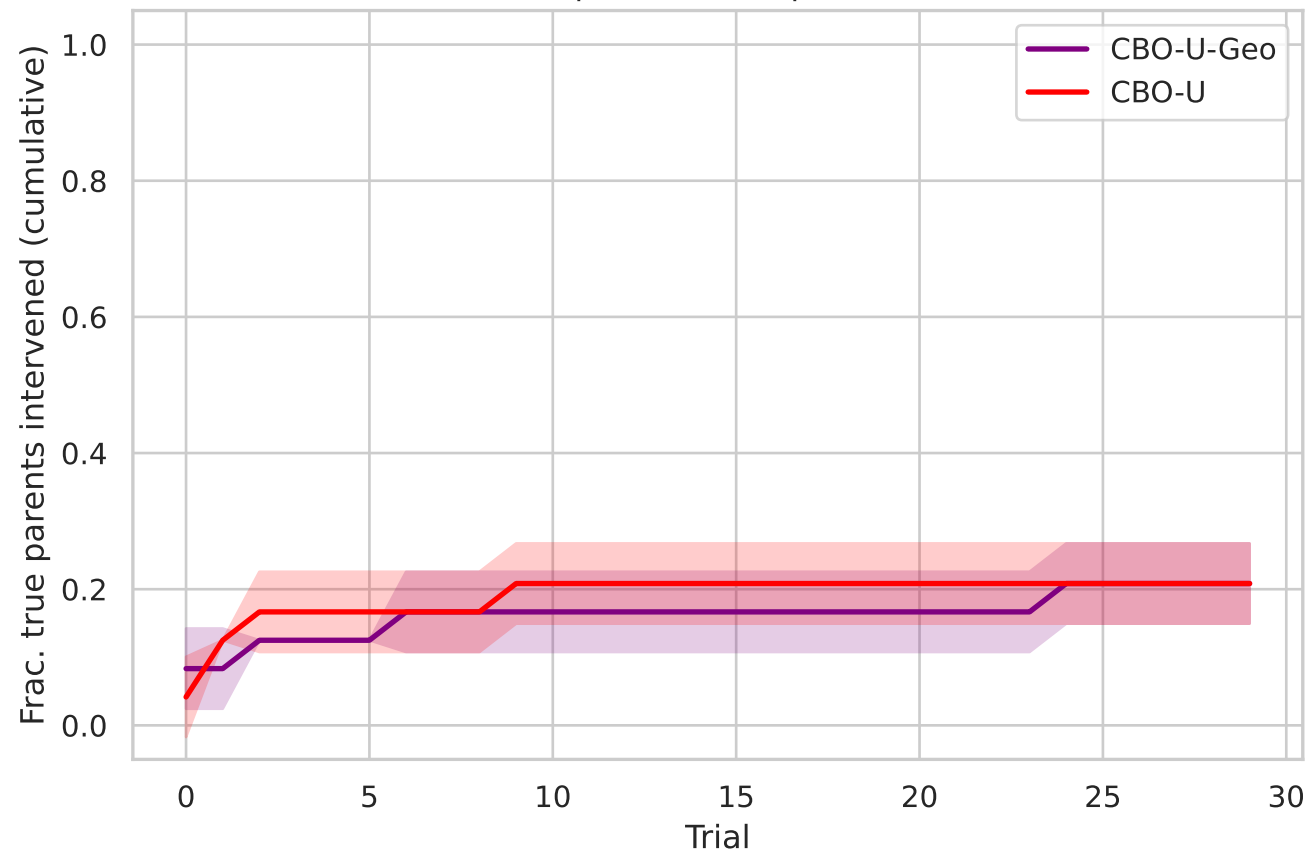
Gwps40 - 8 true parents
