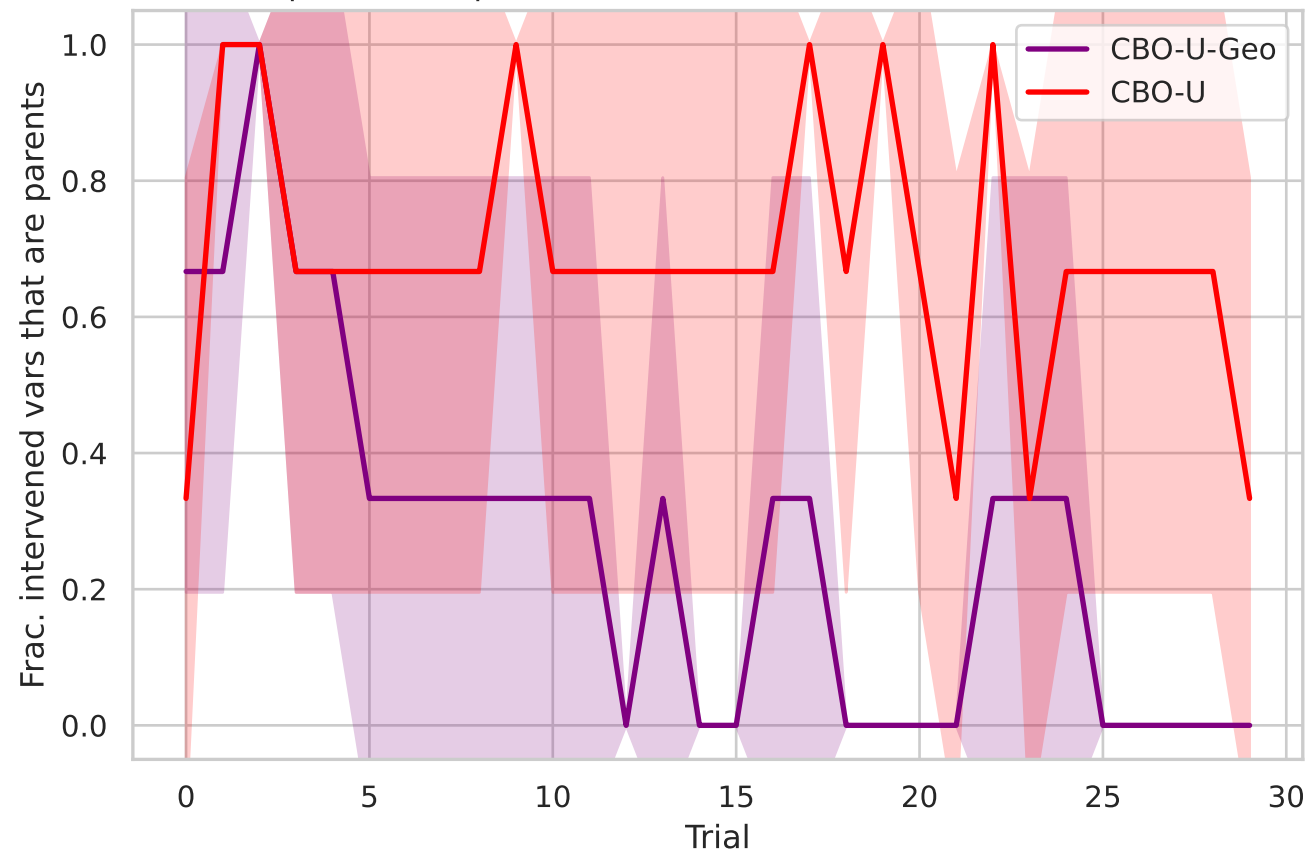
Gwps40 - true parents ['6', '9', '15', '18', '25', '34', '35', '38']
