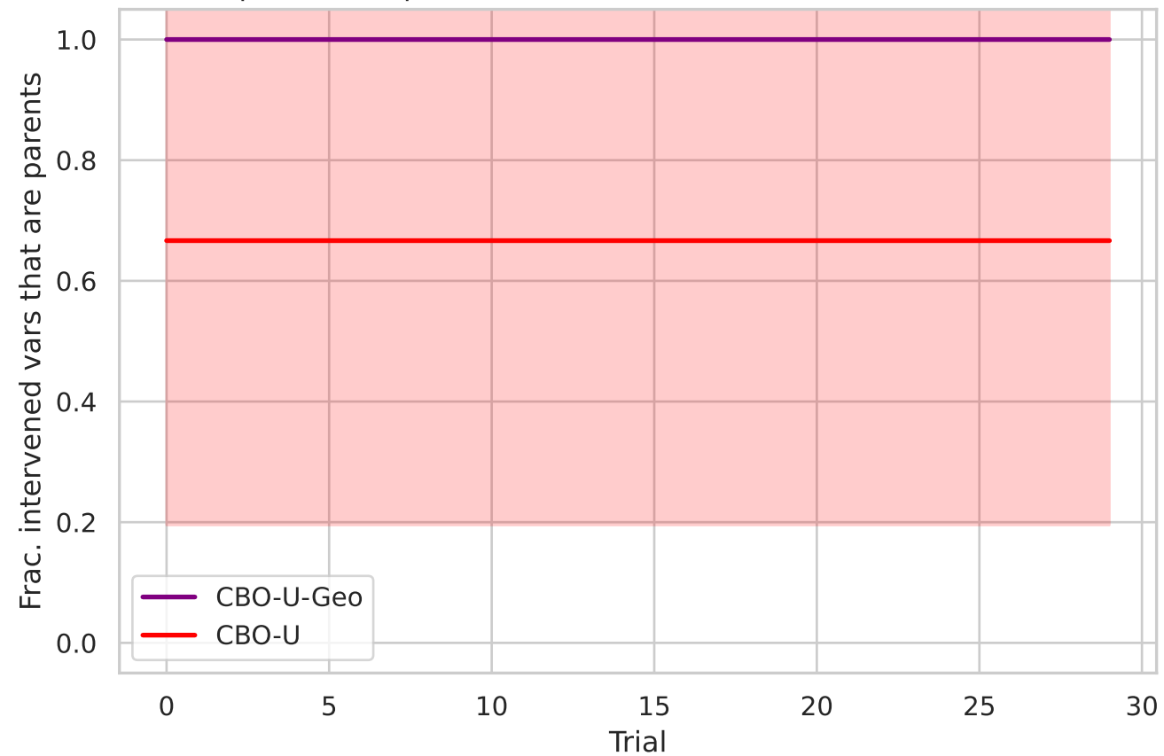
Gwps60 - true parents ['10', '14', '24', '29', '36', '51', '53', '57']
