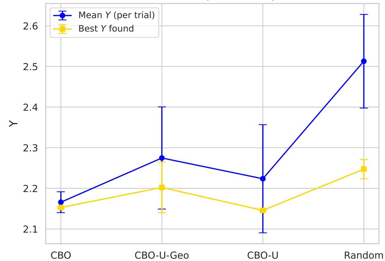
Erdos100 (Nonlinear)
