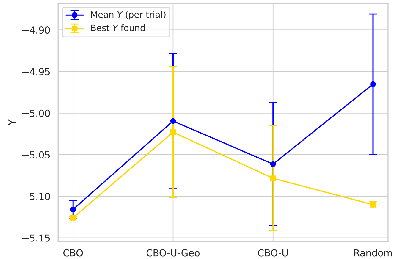
Erdos100 (Nonlinear)
