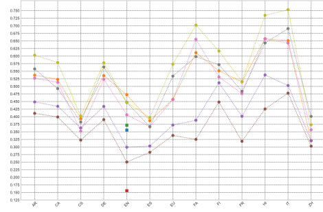
Figure 2: IoU Scores for Models trained on synthetic data and multiple validation sets.
