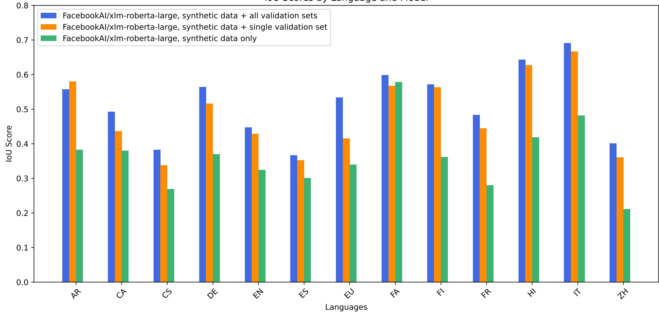
IoU Scores by Language and Model
