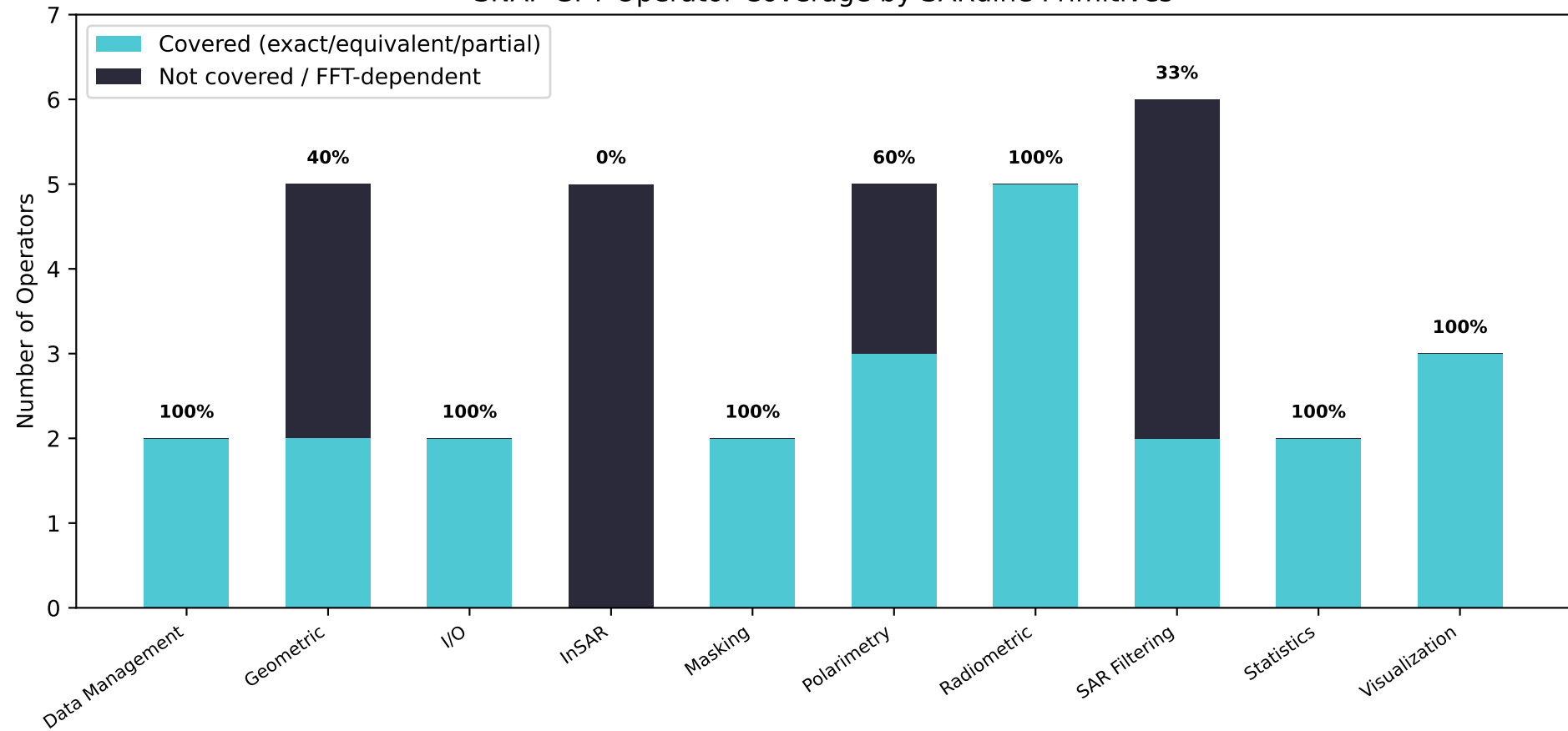
SNAP GPT Operator Coverage by SARdine Primitives
