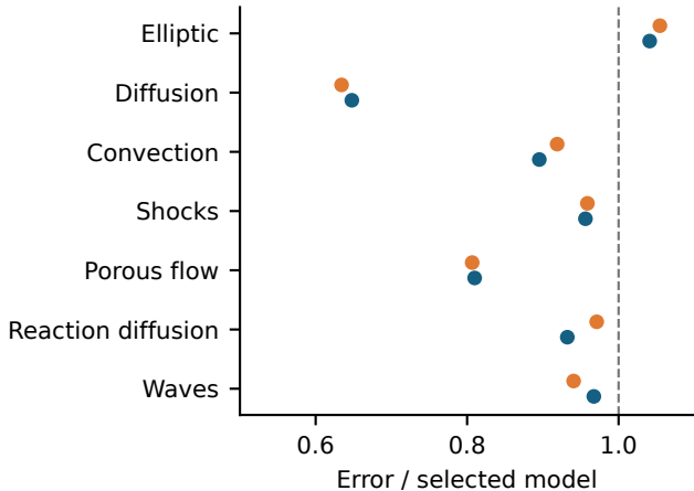
(a) Class level results, K = 5
