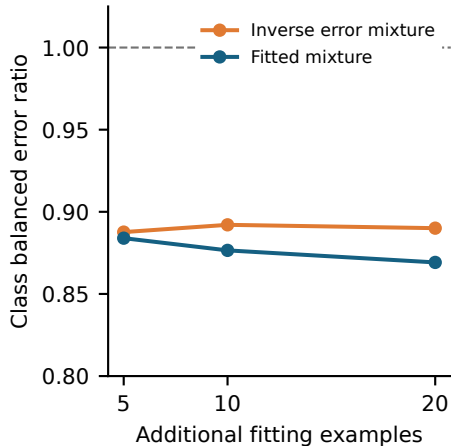
(b) Fitting budget
