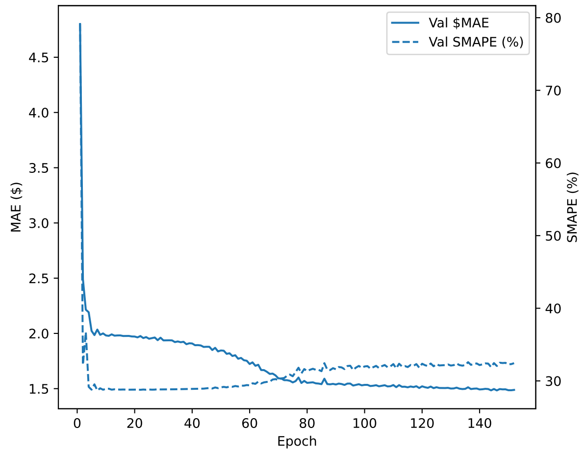
Validation error (dollars) and SMAPE (%)
