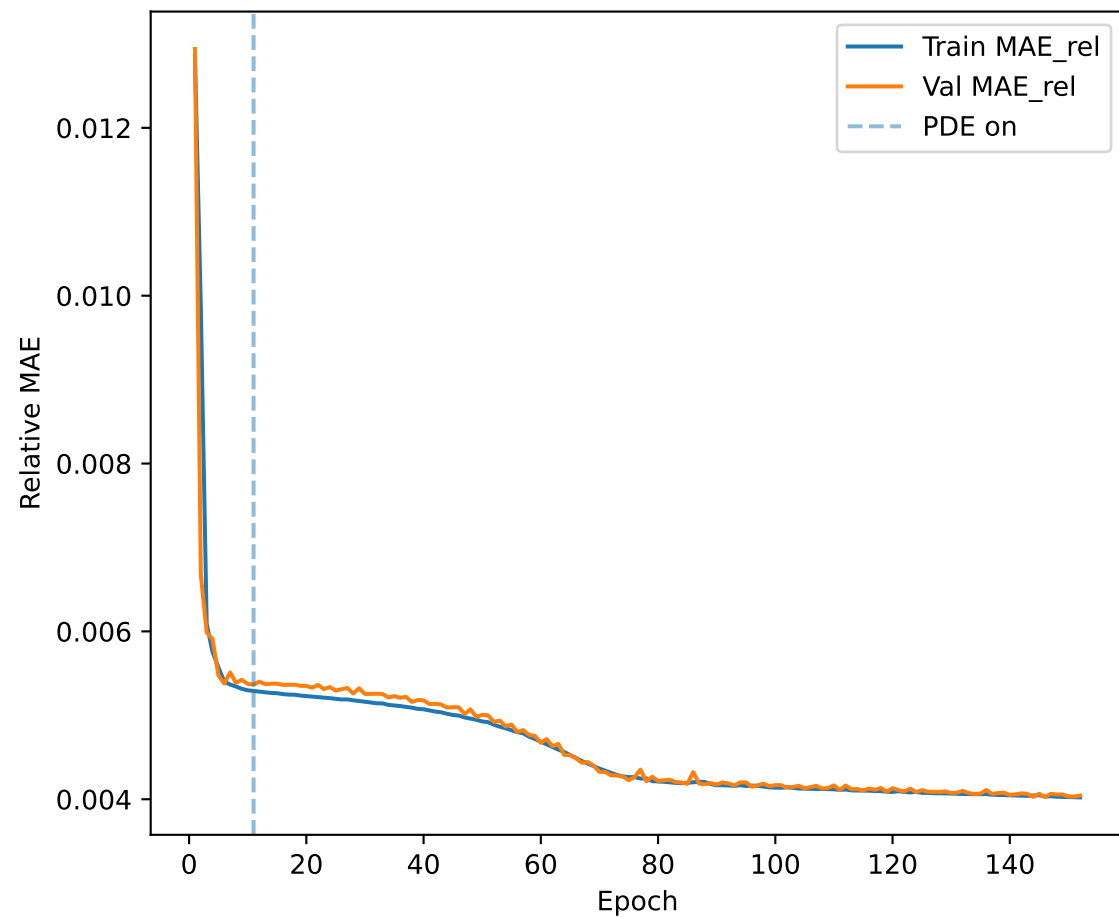
Loss — Train vs Val
