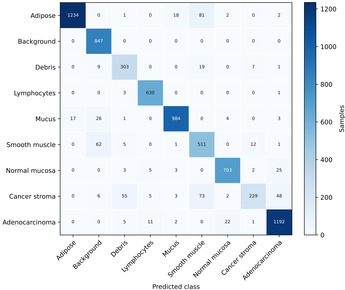
Official ResNet-50 PathMNIST Test Confusion Matrix
