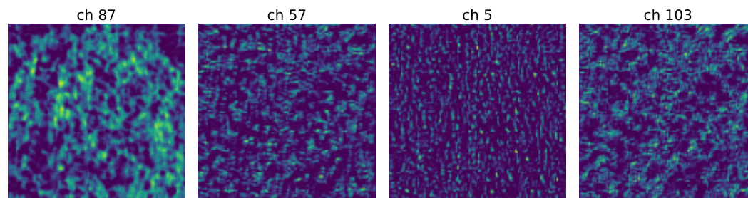
Convolutional layer 2
