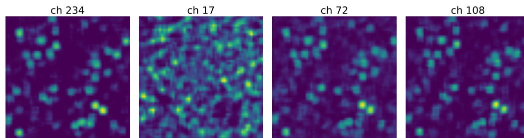
Convolutional layer 3
