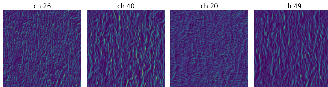
Convolutional layer 1
