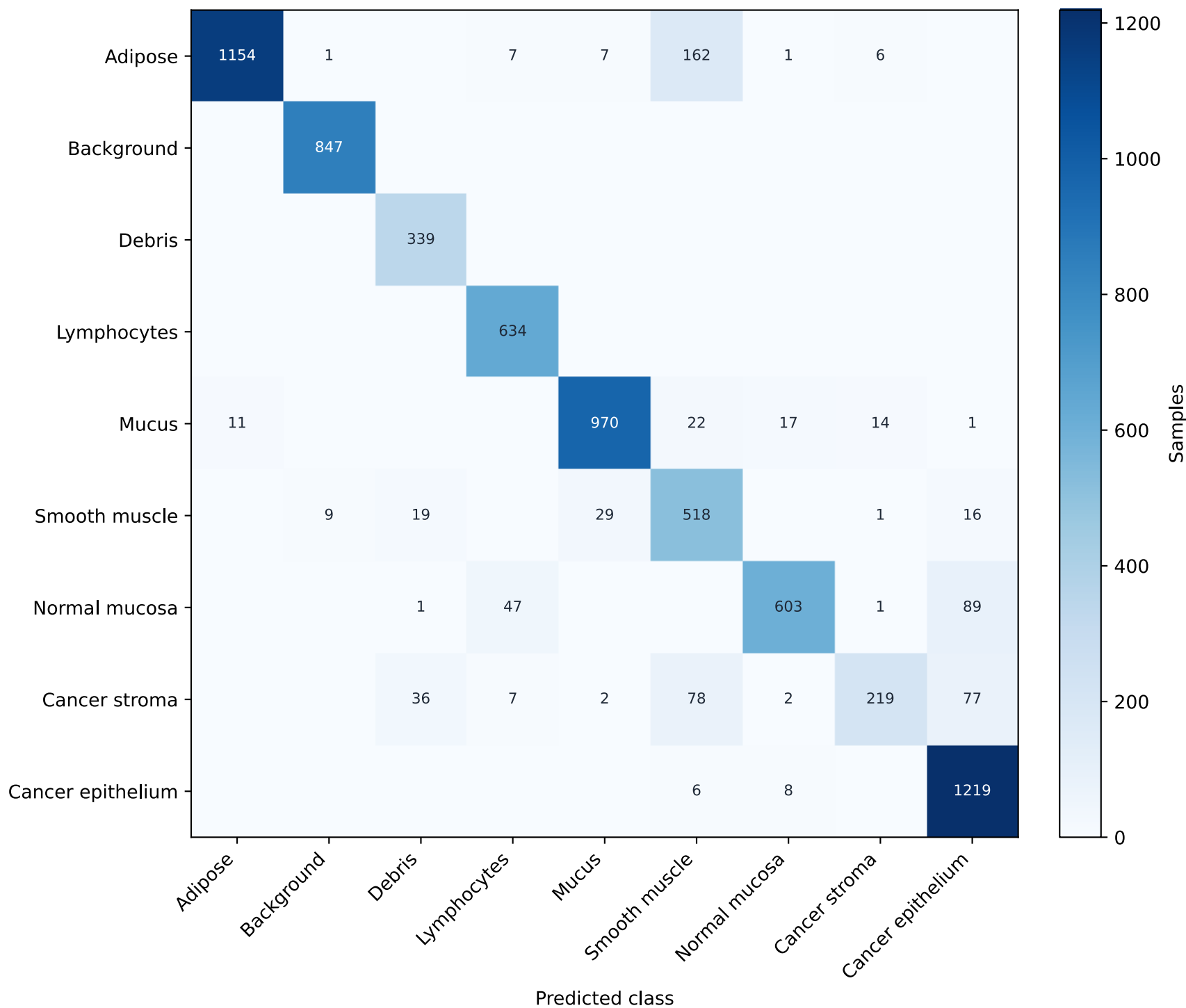
Baseline 224 Test Confusion Matrix
