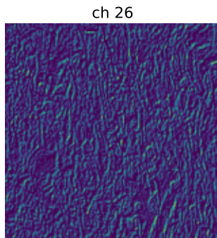
Convolutional layer 1
