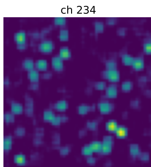
Convolutional layer 3
