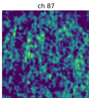
Convolutional layer 2
