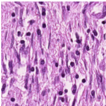
Input patch
