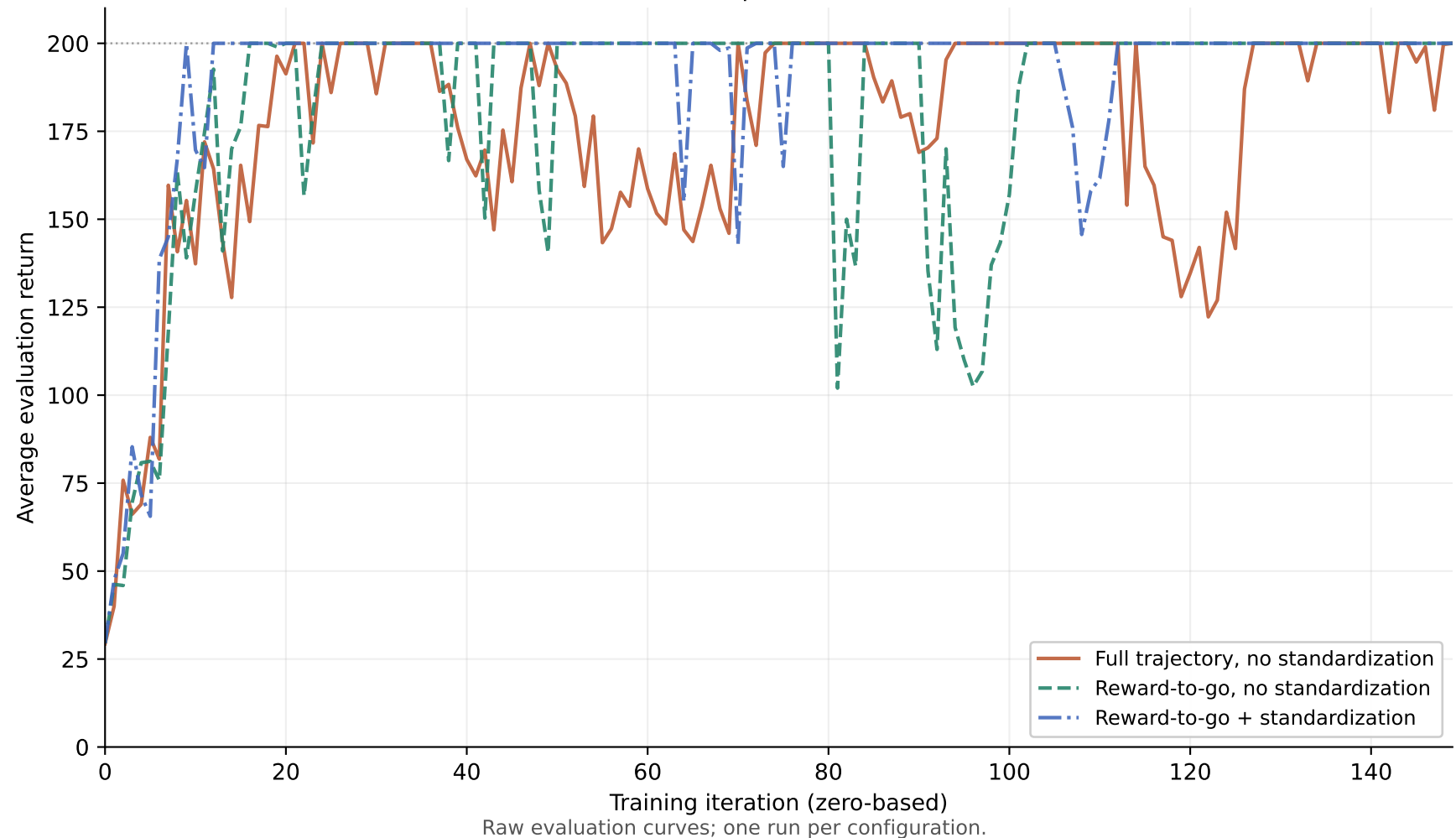
CartPole-v0 | batch size 6,000
