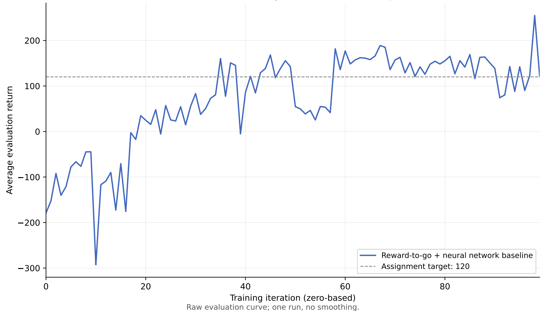
LunarLanderContinuous-v2 | batch 10,000, learning rate 0.005
