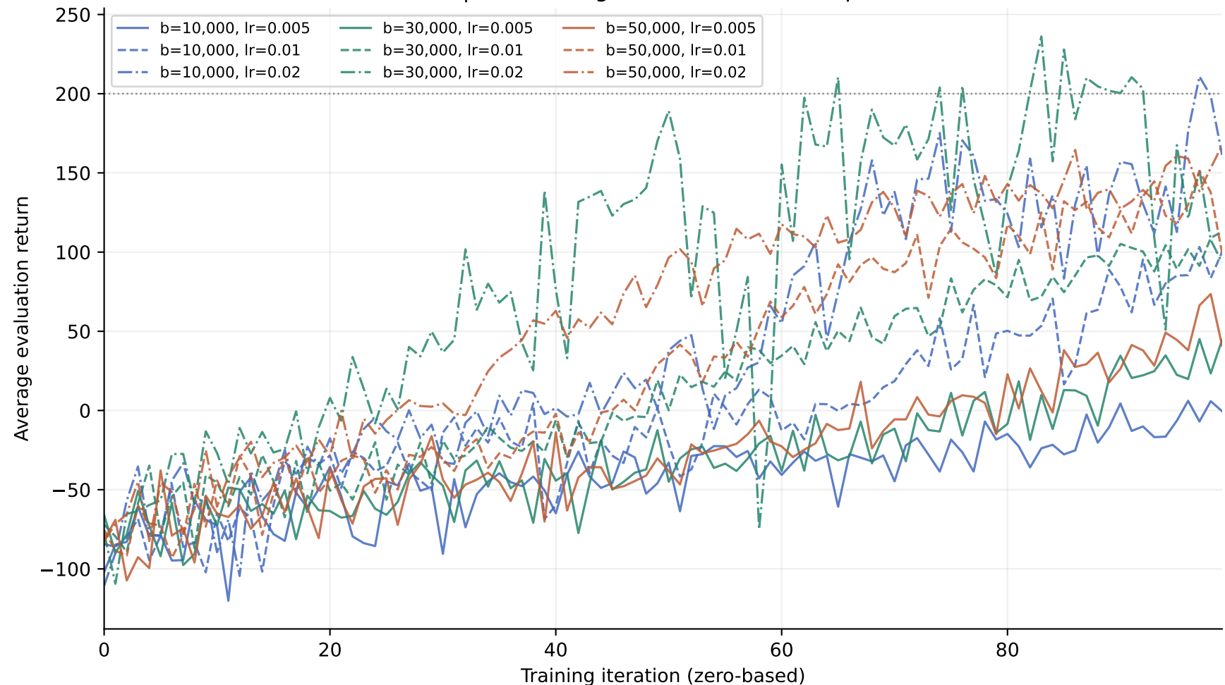
HalfCheetah-v4 | reward-to-go + neural baseline: parameter search
