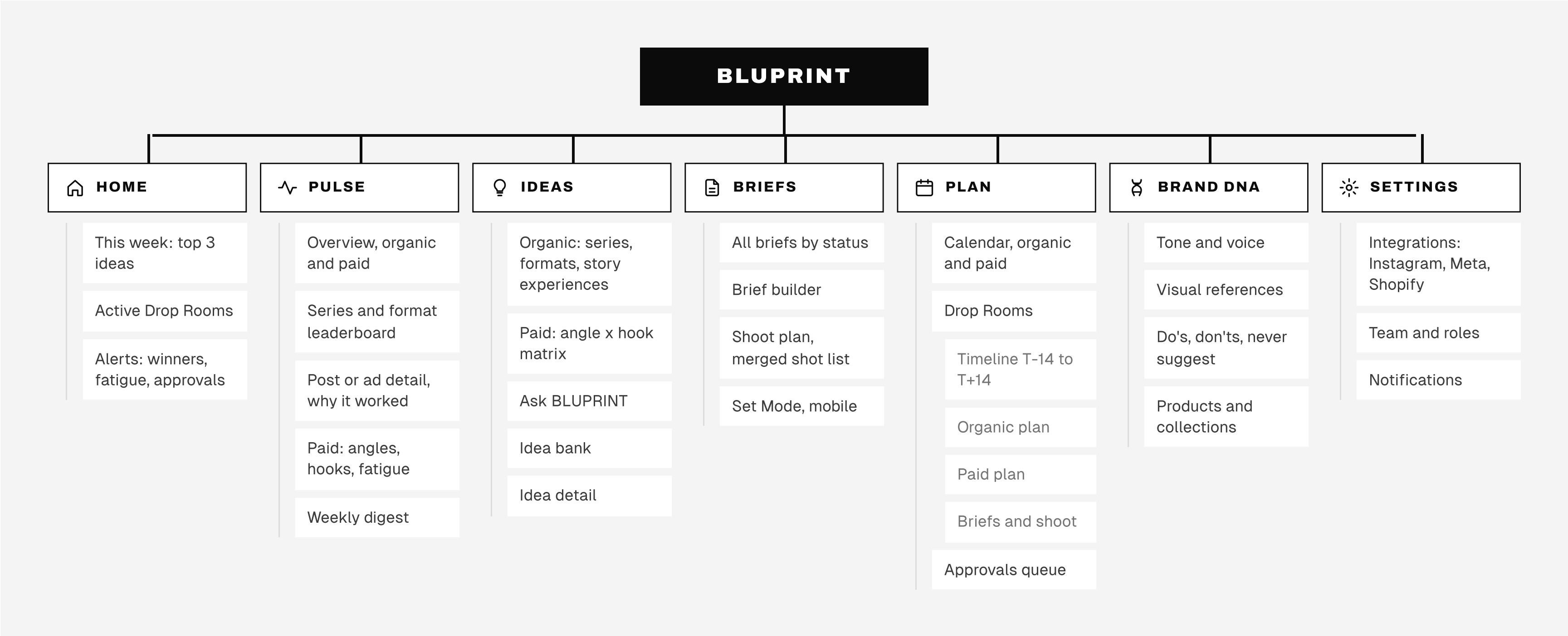
SITEMAP, WEB APP
