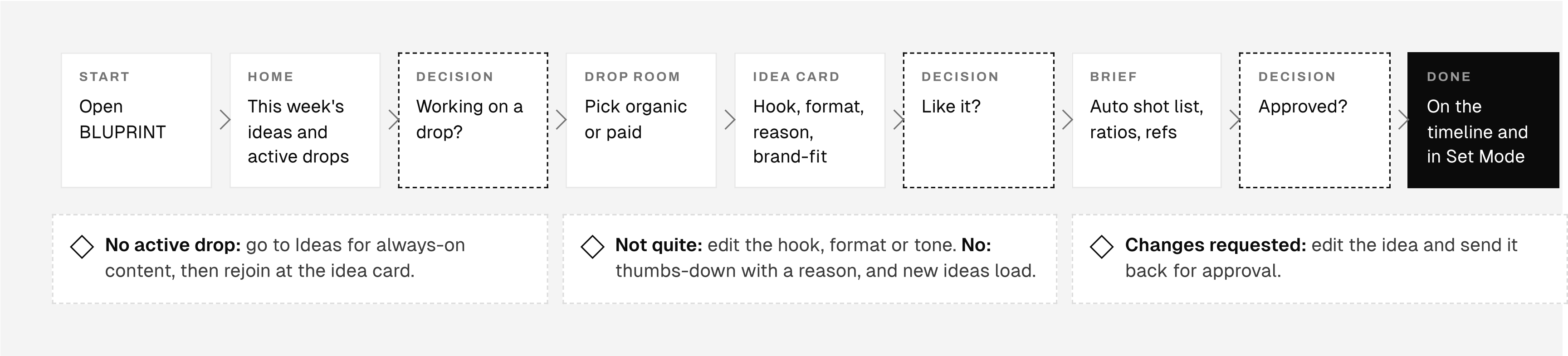
PRIMARY USER FLOW
