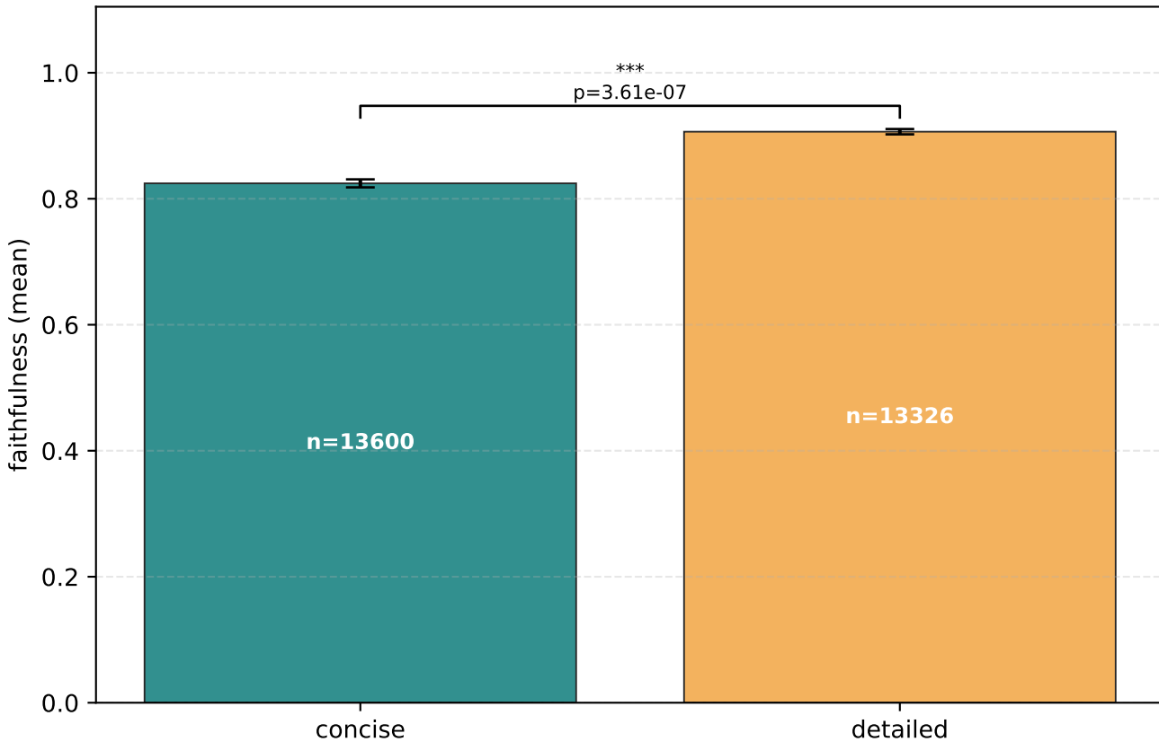
RAGAS faithfulness by prompt template (mean with bootstrap 95% CI, n = per-question scores)
