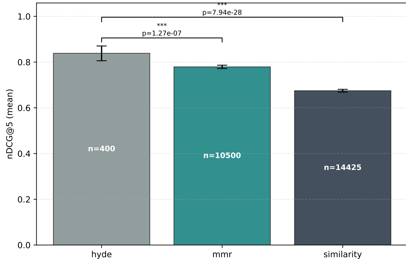
nDCG@5 by retrieval strategy (mean with bootstrap 95% CI, n = per-question scores)
