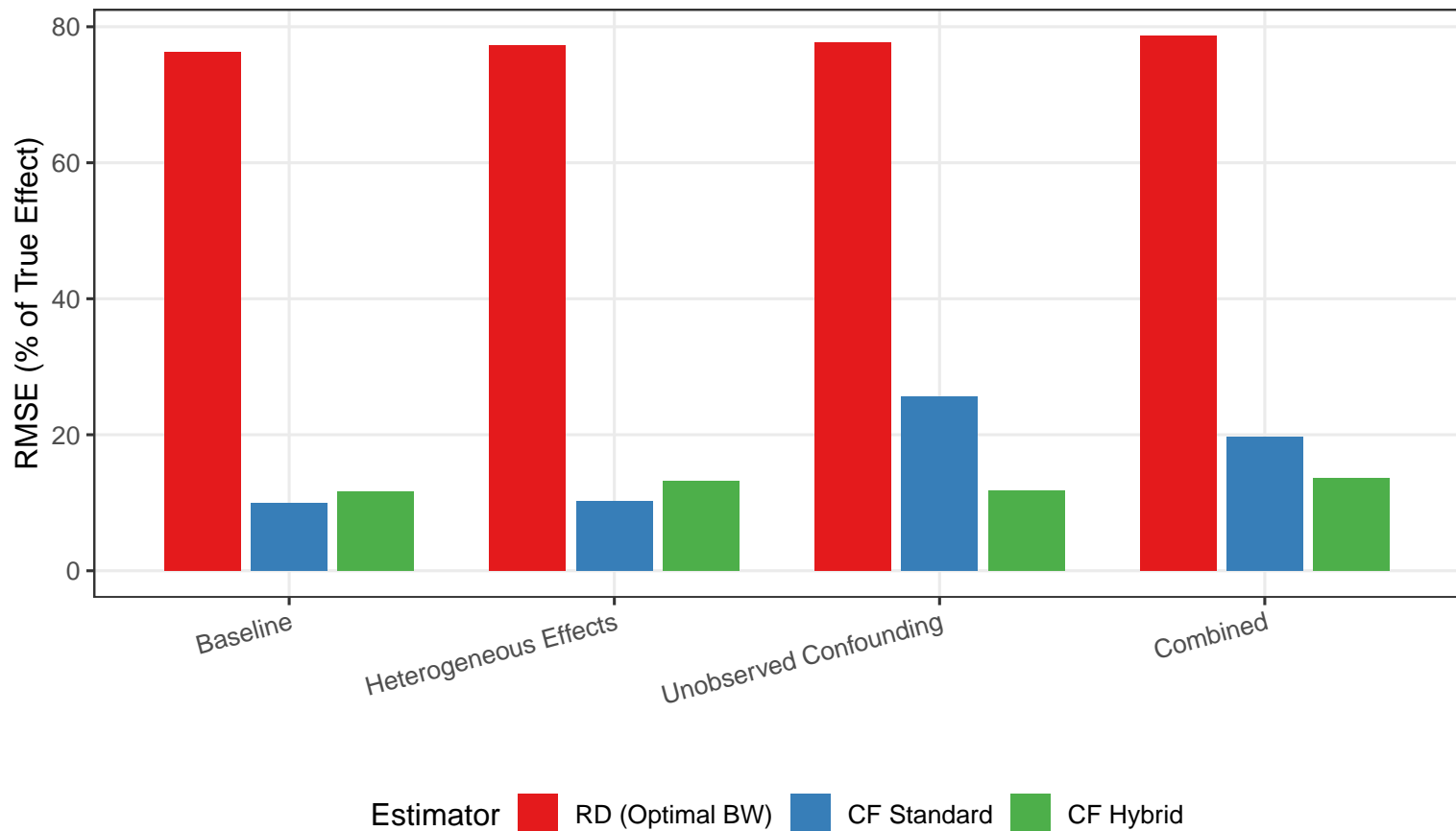
Root Mean Squared Error by Estimation Method and Scenario
