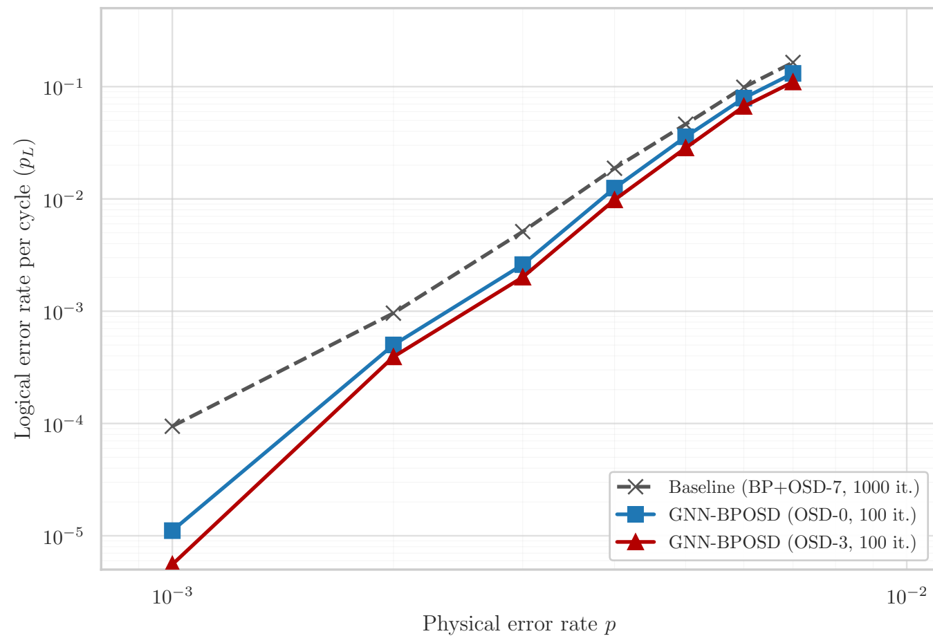
Bivariate Bicycle [[72,12,6]]
