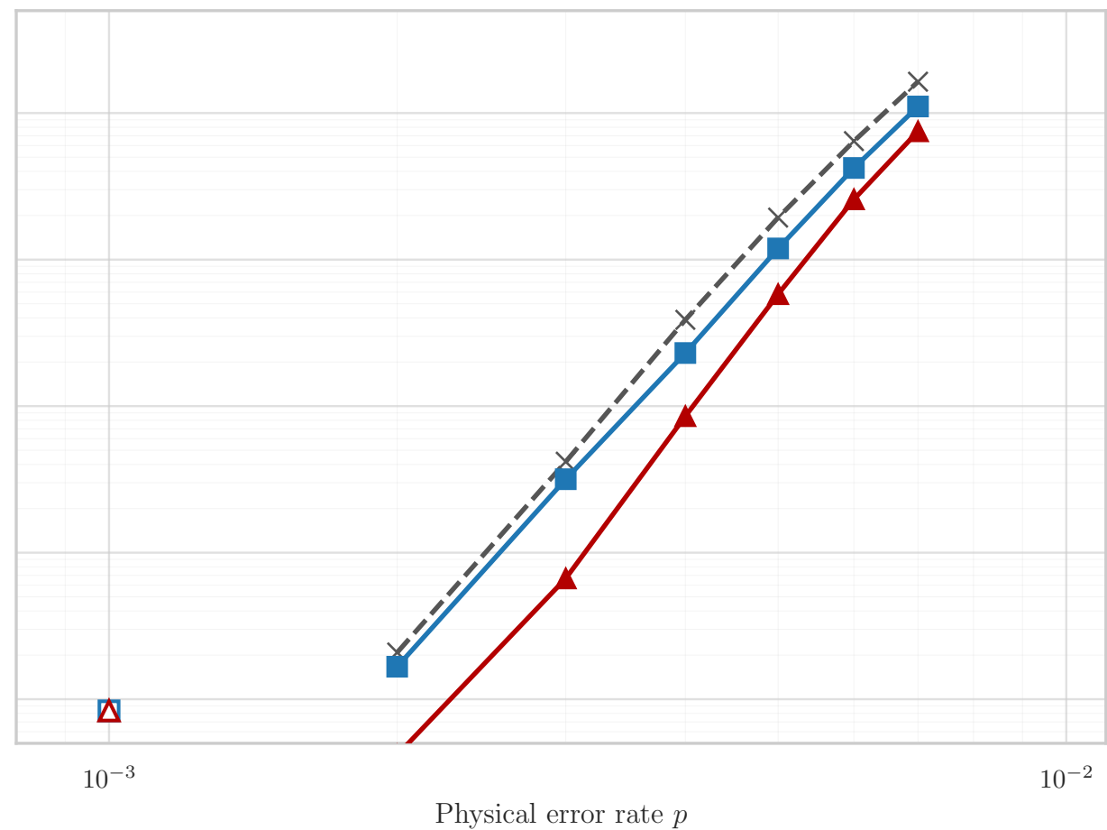
Bivariate Bicycle [[144,12,12]]
