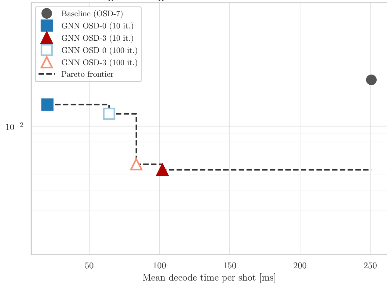
[[144,12,12]] Pareto Trade-off at p = 0.005
