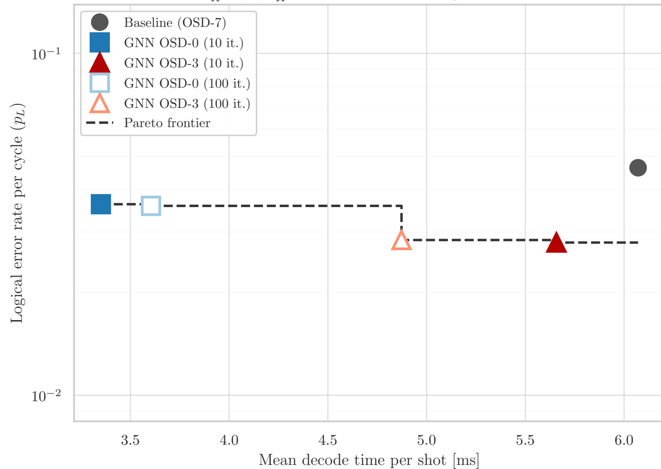
[[72,12,6]] Pareto Trade-off at p = 0.005
