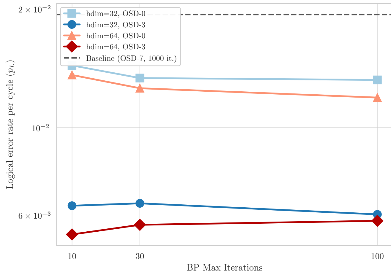
[[144,12,12]]: Accuracy vs Iterations ( p = 0.005 )
