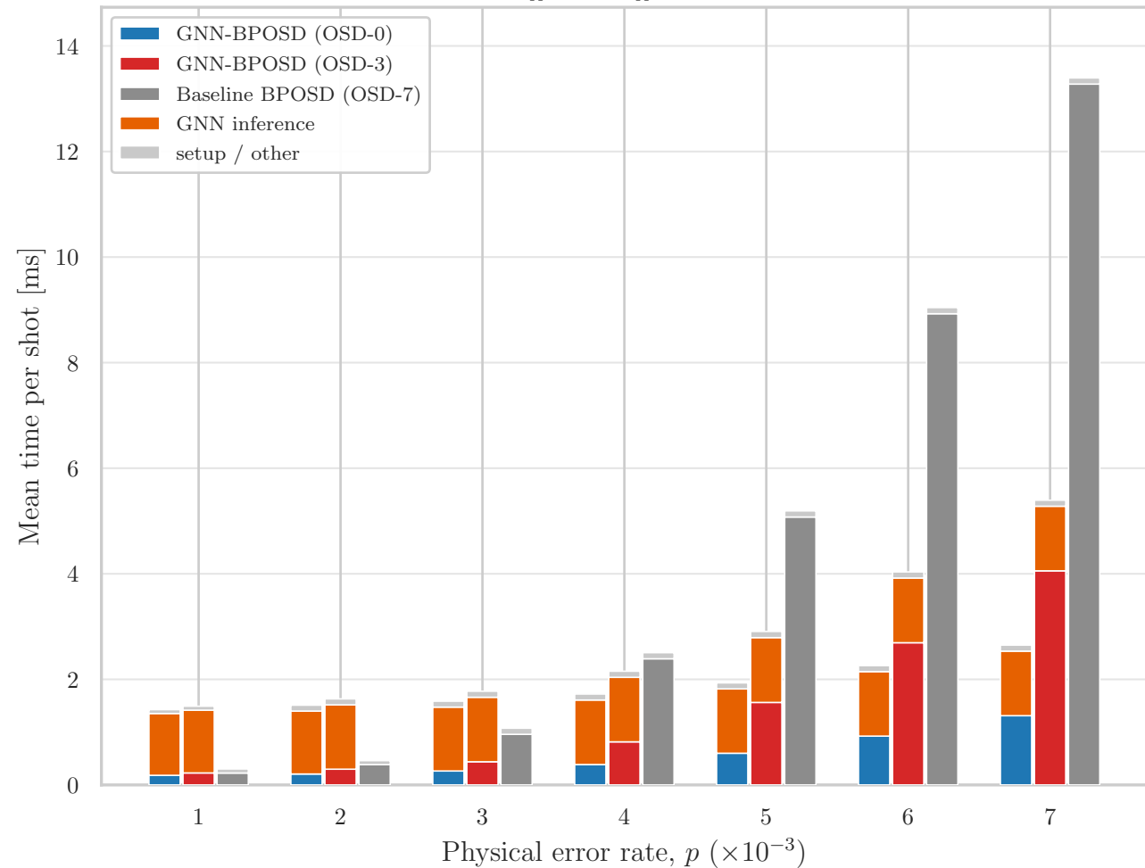
[[72,12,6]] code
