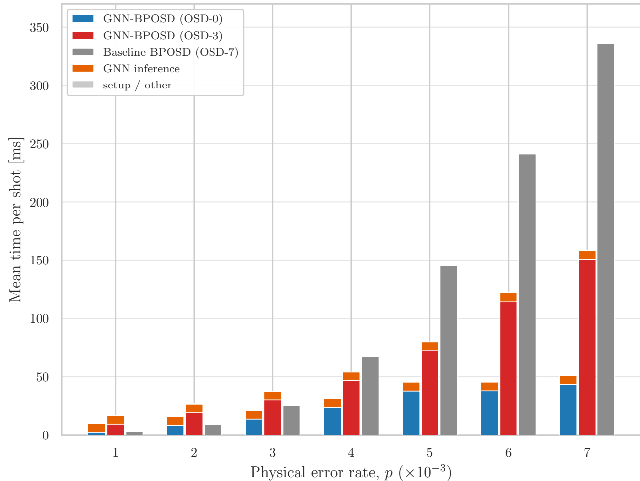
[[144,12,12]] code
