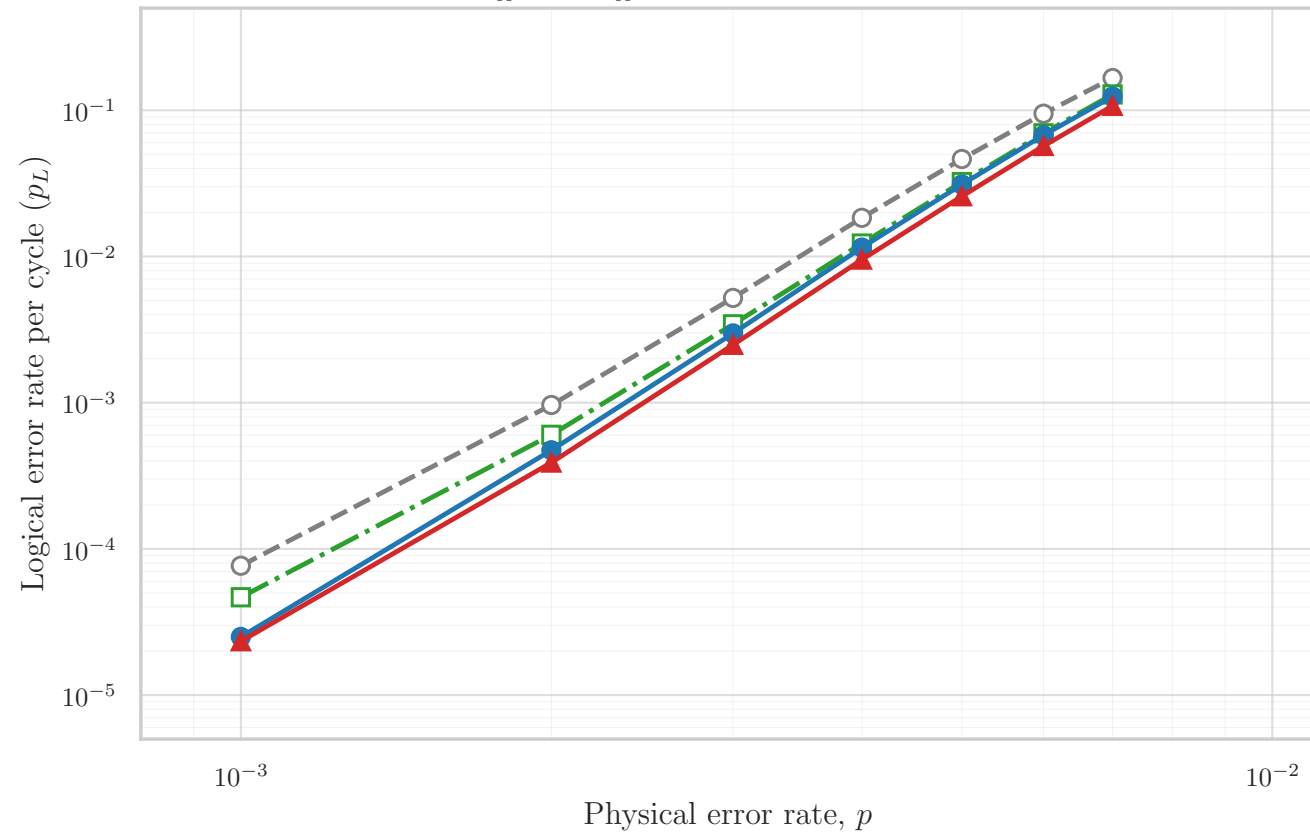
[[72,12,6]] Decoder Performance
