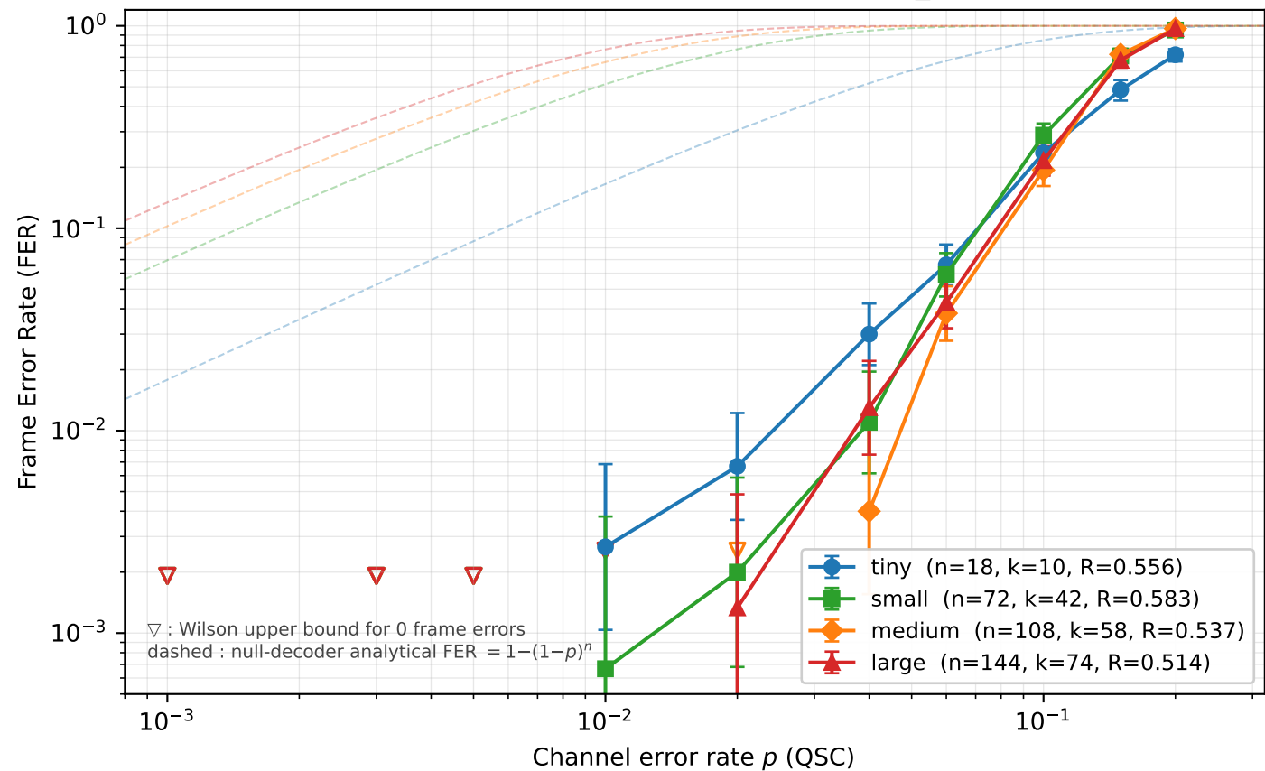
BP-FFT decoder, F_4 -linear BB codes (max_iters=50)
