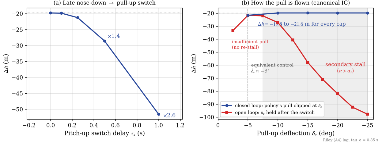
Fig. 9 Sensitivity of the recovery to pilot execution errors at the canonical IC. (a) Delaying the nose-down → pull-up switch by \tau_s , with the loss multipliers annotated. (b) The pull phase flown in its two modes, on one signed deflection scale (axis inverted so that pulling harder reads rightward): closed loop (blue), the policy with its pull commands clipped at \delta_e ; open loop (red), the same deflection held constant after the switch. Dotted line: the optimal loss; dashed vertical: the equivalent control \bar{\delta}_e \approx -5^\circ ; shaded: the held pulls that re-stall the wing ( \alpha > \alpha_s ). Note that the abscissa means a different thing for each curve: the deflection actually flown for the open loop, only a ceiling for the closed loop.
