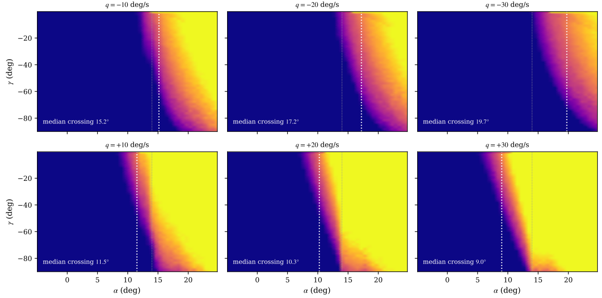
Fig. 5 The commanded-elevator policy over the (\alpha, \gamma) plane at V/V_s = 0.9 , at nose-down (top row) and nose-up (bottom row) pitch-rate slices; the q = 0 slice, with its crossing at 13.4^\circ , is in Fig. 3. The white dotted line travels with each slice’s median crossing (elevator zero crossing over the recovery-relevant columns, -40^\circ \leq \gamma \leq 0 , V \leq 1.2 V_s ); the faint one is fixed at \alpha_s = 14^\circ . The pull/push boundary shifts by about 2^\circ per 10 deg/s of pitch rate: with nose-down rotation in hand the optimum reverses at higher angle of attack, with nose-up rotation it pushes earlier. The tilt is the momentum anticipation of the reversal, and reconciles the q = 0 maps with the closed-loop reversal statistics of Table 5, flown at q \approx -20 deg/s.
