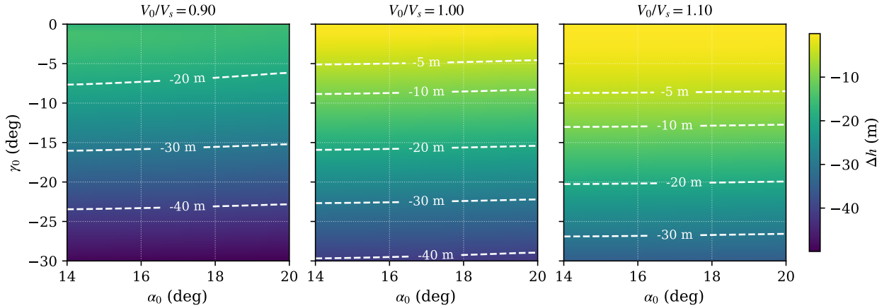
Fig. 7 Altitude loss of the exact optimum over the stalled-entry plane ( \alpha_0 abscissa, \gamma_0 ordinate, q_0 = 0 ), at the stalled-entry airspeeds of the policy maps of Fig. 6; one closed-loop rollout per node on a 31 \times 25 grid, labeled contours on a shared scale. The field is governed by \gamma_0 (a 35 m span at 0.90 V_s , 41 m at V_s ) and only weakly by \alpha_0 (under 2 m across the entire stalled range).
