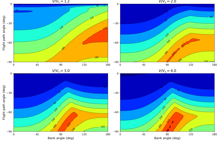
Fig. 1 Contour plots of minimal altitude loss ( \Delta h_{min} \approx -V^* ) during aircraft pullout maneuvers, evaluated on the baseline 53,280-state grid. Each subplot presents the altitude loss across the bank angle ( \mu_0 ) and flight path angle ( \gamma_0 ) envelope for a fixed initial airspeed ( V_0/V_s ). The global topology of the solution perfectly aligns with established literature [7], validating the accuracy of the on-the-fly RK4 integration and the consistency of the barycentric interpolator.
