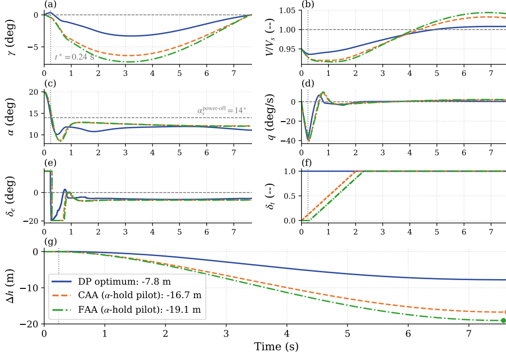
Fig. 9 Time-domain comparison at the canonical deep-stall initial condition: exact DP policy (blue, solid) vs. the scripted CAA (orange, dashed) and FAA (green, dash-dotted) procedures of Table 7. Panel (f) isolates the protocol difference: instantaneous full power (DP), 2 s ramp from t = 0 (CAA), ramp from the unstall event (FAA); final losses in panel (g). The vertical dotted line marks the DP policy’s elevator-switch instant t^* \approx 0.24 s, the reference event for the pilot-error study of Sec. V.H. Both scripted pilots are held to the same pull authority as the optimum ( \delta_e \geq -19.69^\circ at this entry), so the figure isolates the timing of the power application rather than confounding it with how hard the pilot hauls back. The DP traces execute the policy through the barycentric action blend of Sec. V.C; the intermediate deflections and throttle settings of panels (e)–(f) are convex combinations of the discrete extremes, not commands the optimizer selected: the underlying policy is bang-bang, and holds full throttle throughout. The brief \gamma > 0 excursion of the optimum (panel a) is the transient derived in Appendix B. The dashed line in panel (c) is the power-off stall boundary of the Riley tables, \alpha_s = 14^\circ ; the superscript qualifies the boundary, not the state of the aircraft, which holds full throttle throughout. Under power the lift curve continues to rise past that value, so the optimum’s excursion above the line is not a re-stall.
