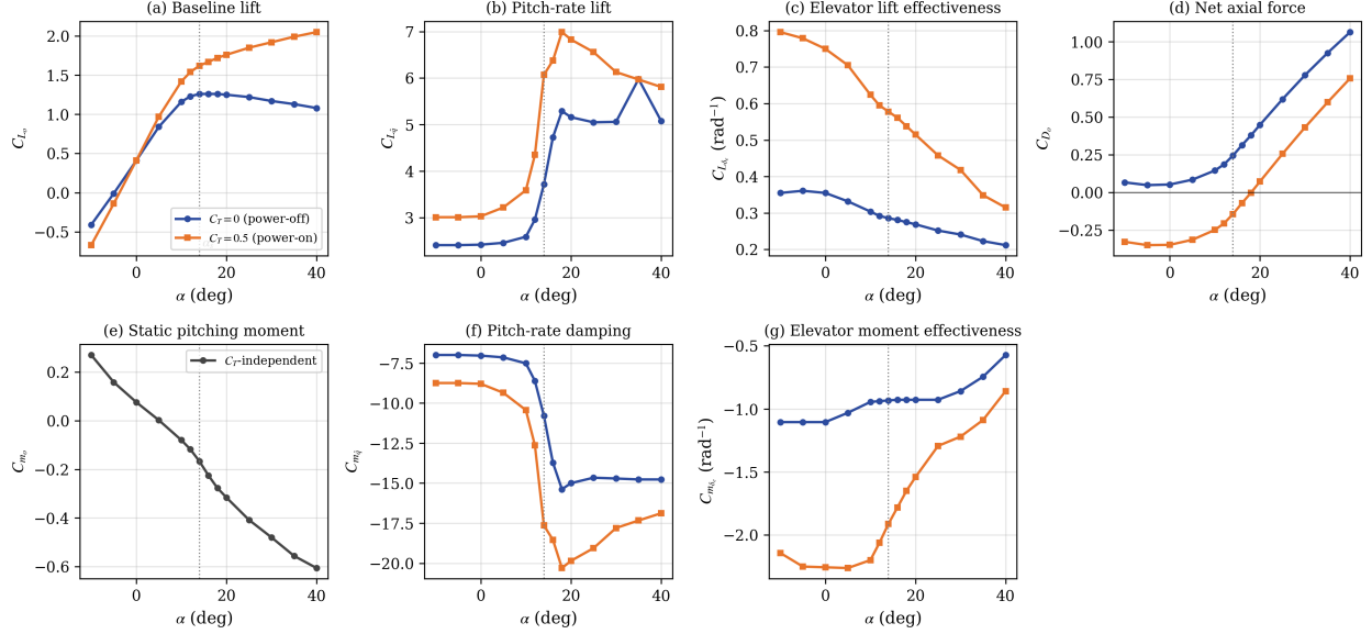
Fig. 5 The seven Riley (1985) Table III coefficients vs. angle of attack at the two tabulated propulsive conditions (one panel per table of Appendix A; C_{m_0} is C_T -independent). Three features drive the recovery physics: (a) baseline lift C_{L_0} shows the power-off flat-top stall plateau vs. monotone power-on growth from slipstream augmentation; (d) the negative power-on values of the net axial-force coefficient C_{D_0} are the embedded-thrust fingerprint of Eq. (15); (f) pitch-rate damping C_{m_q} more than doubles across the stall. The dotted line marks the stall angle \alpha_s = 14^\circ .
