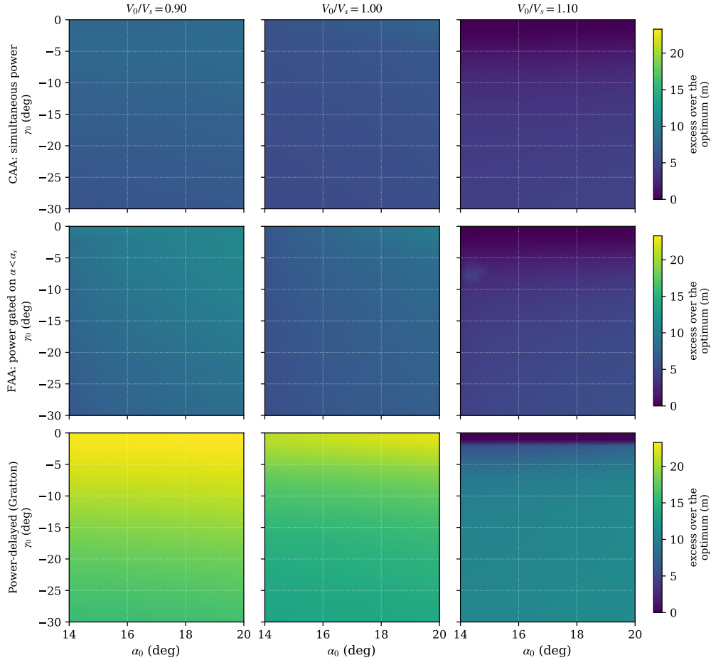
Fig. 8 Excess altitude loss of each recovery procedure over the optimum of Fig. 7, \Delta h_{\text{opt}} - \Delta h_{\text{proc}} , from the same entries; all arms fly the DP-optimal elevator schedule, so power timing is the only difference between rows. Top: CAA, full power from t = 0 through a 2 s ramp: the floor imposed by the engine itself. Middle: FAA, power gated on \alpha < \alpha_s , then the same ramp: the floor plus the doctrine penalty, largest toward low-speed, shallow entries. Bottom: Gratton's power-delayed protocol (2 s pause, then the ramp). The three rows repeat one shared viridis scale anchored at zero excess, so the ranking reads directly down each column. On every one of the 1550 nodes shown, the ordering optimum \leq CAA \leq FAA \leq PD holds without exception.
