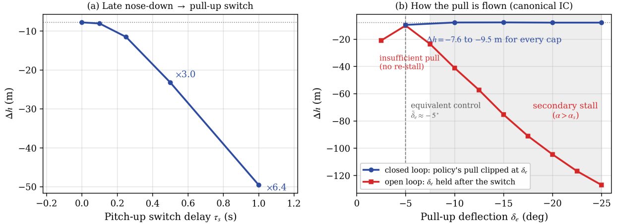
Fig. 12 Sensitivity of the recovery to pilot execution errors at the canonical IC. (a) Delaying the nose-down \rightarrow pull-up switch by \tau_s , with the loss multipliers annotated. (b) The pull phase flown in its two modes, on one signed deflection scale (axis inverted so that pulling harder reads rightward): closed loop (blue), the policy with its pull commands clipped at \delta_e ; open loop (red), the same deflection held constant after the switch. Dotted line: the optimal loss; dashed vertical: the equivalent control \bar{\delta}_e \approx -5^\circ ; shaded: the held pulls that re-stall the wing ( \alpha > \alpha_s ). Note that the abscissa means a different thing for each curve: the deflection actually flown for the open loop, only a ceiling for the closed loop.
