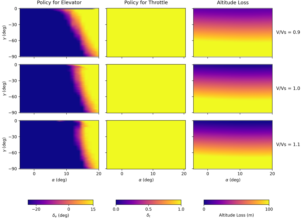
Fig. 6 Exact DP heatmaps for the 4-DOF symmetric stall recovery with the Riley (1985) propulsion-coupled aerodynamic model: optimal commanded elevator ( \delta_e^* ), throttle ( \delta_t^* ), and the value function read as minimum altitude loss, -V(x) , over the evaluated flight envelope (slice q = 0 ). -V is the solver’s cost-to-absorption, not the closed-loop metric of the tables and trajectory figures, which execute the blended policy under the dive-and-return rule; the two agree in structure and differ in level by 1–3 m (see text). The elevator panels plot the raw arg max, so the narrow bands of saturated command that appear near \gamma \approx 0 should be read as the switching surface itself rather than as physical reversals: sampling the one-step Q across the full elevator range at those cells spreads it by only 0.04 m out of a 16–18 m cost-to-go (0.2%), so the extremum that wins the tie flips between adjacent rows while -V stays smooth. The blend of Sec. V.C, which is what the closed loop executes, averages across those ties.
