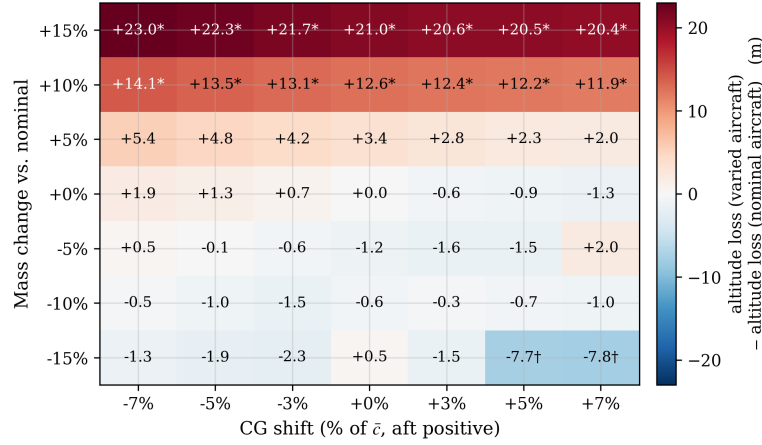
Fig. 10 Excess altitude loss (m) of the nominal policy flown on the perturbed aircraft, relative to the same policy on the nominal aircraft ( -7.80 m, canonical IC), over the mass change ( \pm 15\% of the reference weight) and CG shift ( \pm 7\% of \bar{c} , aft positive) envelope. Positive (red) = additional loss; negative (blue) = less loss than nominal. Rows are read as the weight of the day, columns as its placement. At nominal weight the aft-CG credit is genuine; in the light rows the reported value is the first zero crossing of a sustained oscillation and understates the loss. Asterisks mark the +10 and +15% rows, where the dive is arrested but the aircraft settles into a steady shallow descent and never regains level flight: their values are losses at the 15 s cutoff, and lower bounds. Daggers mark the two cells that reach \gamma = 0 while still stalled; both are analysed in the text.
