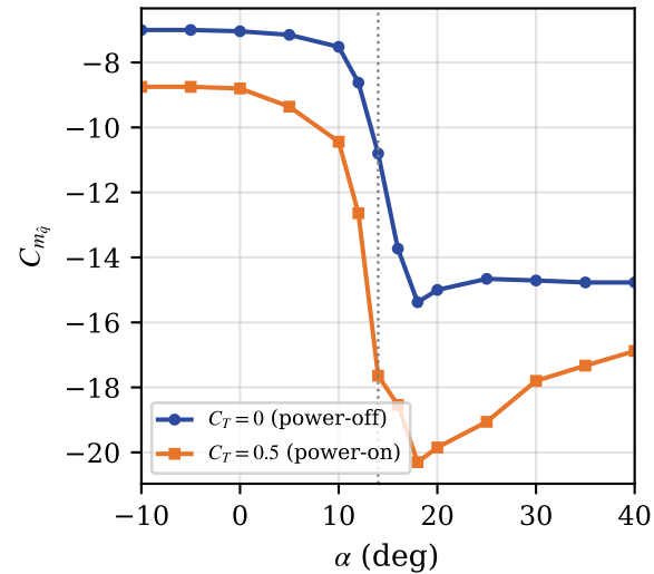
(c) Pitch-rate damping
