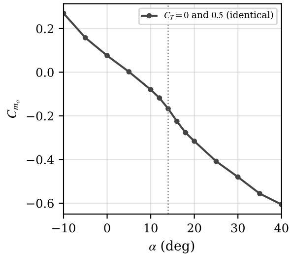
(b) Static pitching moment
