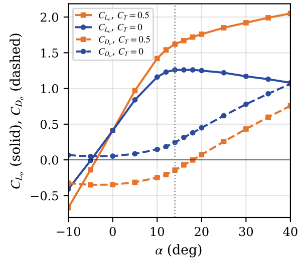
(a) Lift and net axial force
