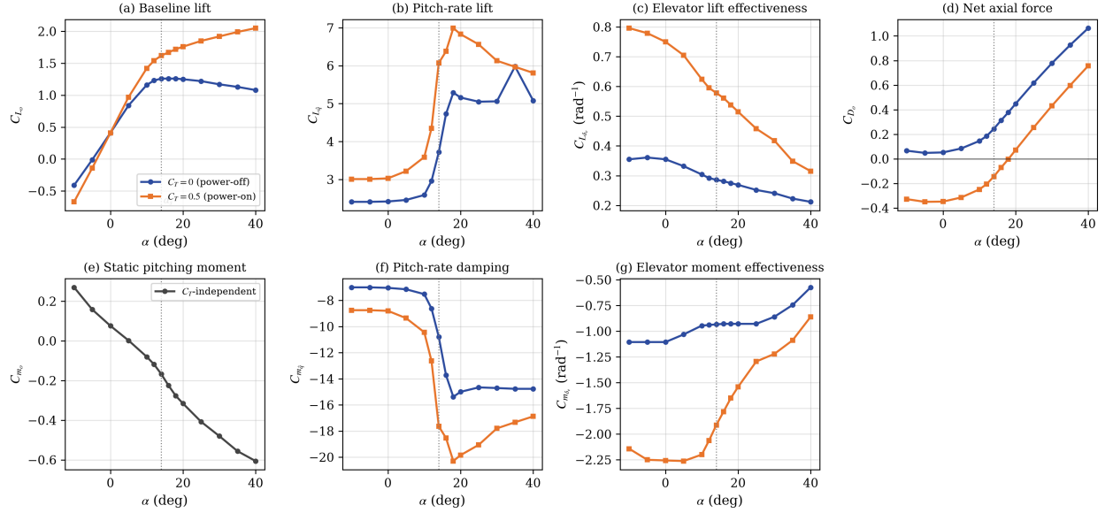
Fig. 4 The seven Riley (1985) Table III coefficients vs. angle of attack at the two tabulated propulsive conditions (one panel per table of Appendix A; C_{m_0} is C_T -independent). Three features drive the recovery physics: (a) baseline lift C_{L_o} shows the power-off flat-top stall plateau vs. monotone power-on growth from slipstream augmentation; (d) the negative power-on values of the net axial-force coefficient C_{D_o} are the embedded-thrust fingerprint of Eq. (15); (f) pitch-rate damping C_{m_q} more than doubles across the stall. The dotted line marks the stall angle \alpha_s = 14^\circ .
