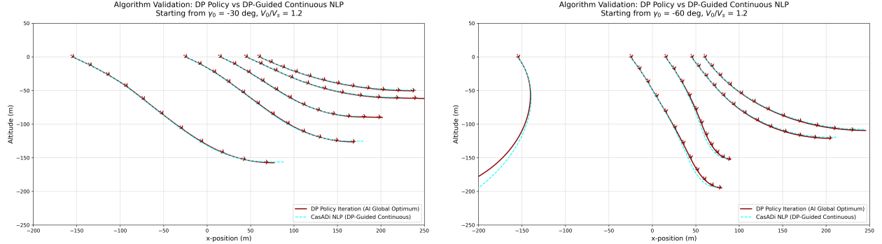
Fig. 13 The closed-loop trajectories behind Table 3: DP rollouts (solid) and DP-guided CasADi/IPOPT solutions (dashed) at \gamma_0 = -30^\circ (left) and \gamma_0 = -60^\circ (right), V_0/V_s = 1.2 , \mu_0 \in \{30, 60, 90, 120, 150\}^\circ . Each arm reconstructs its own horizontal distance from its own integration, so the sub-metre vertical separation between paired curves is not resolved at this scale; the quantitative comparison is between the endpoints at \gamma = 0 , where both arms terminate (Table 3). In the right panel, the leftmost pair is the excluded near-inverted \mu_0 = 150^\circ entry: the policy does not return it to level flight and the NLP did not converge there, so neither curve terminates and their relative position carries no information.
