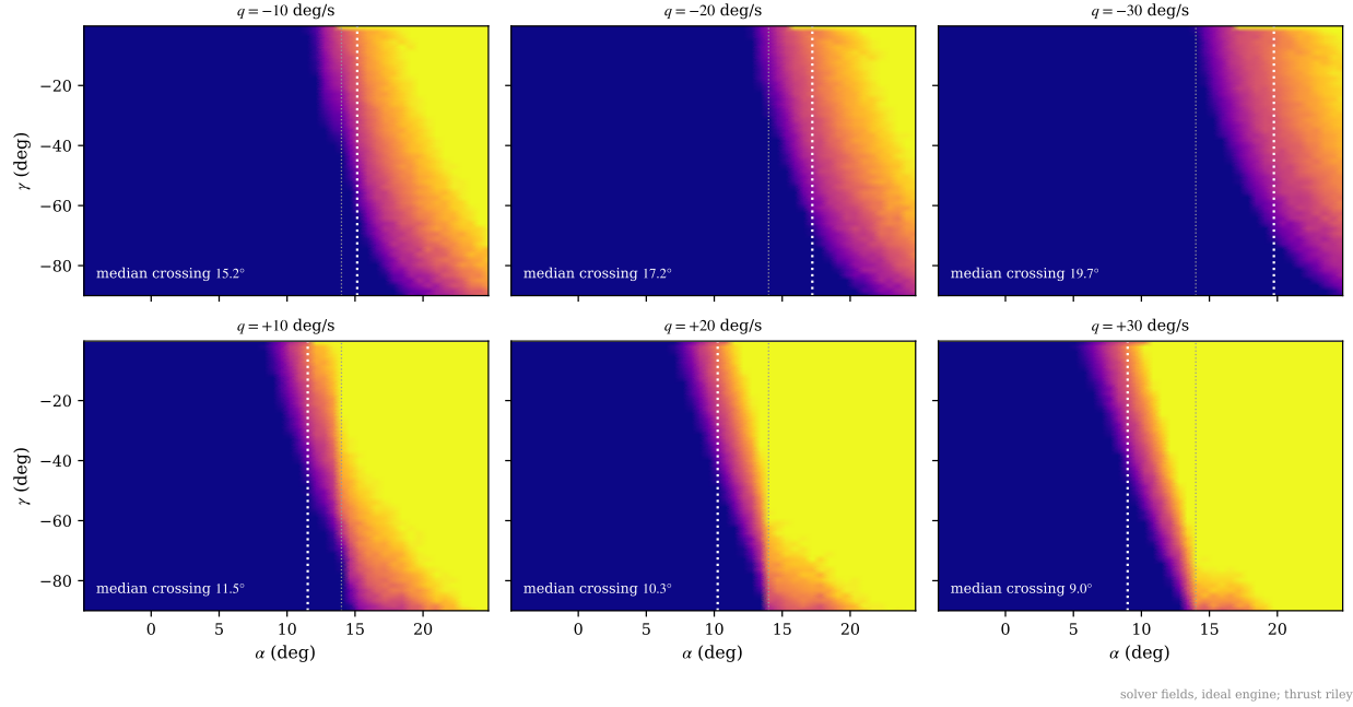
Fig. 14 The commanded-elevator policy over the (\alpha, \gamma) plane at V/V_s = 0.9 , at nose-down (top row) and nose-up (bottom row) pitch-rate slices; the q = 0 slice, with its crossing at 13.4^\circ , is in Fig. 3. The white dotted line travels with each slice’s median crossing (computed as in Sec. V.D); the faint one is fixed at \alpha_s = 14^\circ . The pull/push boundary shifts by about 2^\circ per 10 deg/s of pitch rate: with nose-down rotation in hand the optimum reverses at higher angle of attack, with nose-up rotation it pushes earlier. The tilt is the momentum anticipation of the reversal, and reconciles the q = 0 maps with the closed-loop reversal statistics of Table 5, flown at q \approx -20 deg/s.
