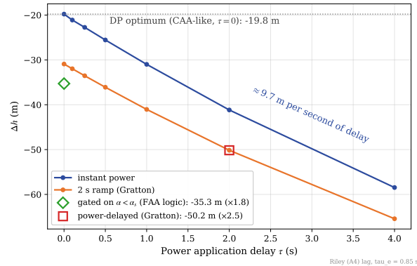
Fig. 9 The power axis: altitude loss vs. power-application delay \tau at the canonical initial condition ( \alpha_0 = 20^\circ , V_0 = 0.95 V_s ), with the optimal elevator schedule held fixed, for the instantaneous and 2 s-ramp power models. The dotted line marks the DP optimum ( \tau = 0 , CAA-like simultaneous power); the diamond, the gated variant (idealized FAA logic); the square, Gratton’s power-delayed protocol ( \tau = 2 s delay plus 2 s ramp). The loss grows monotonically, by \approx 7.7 m per second of delay: the linear reference against which the two pitch axes of Fig. 10 should be read.
