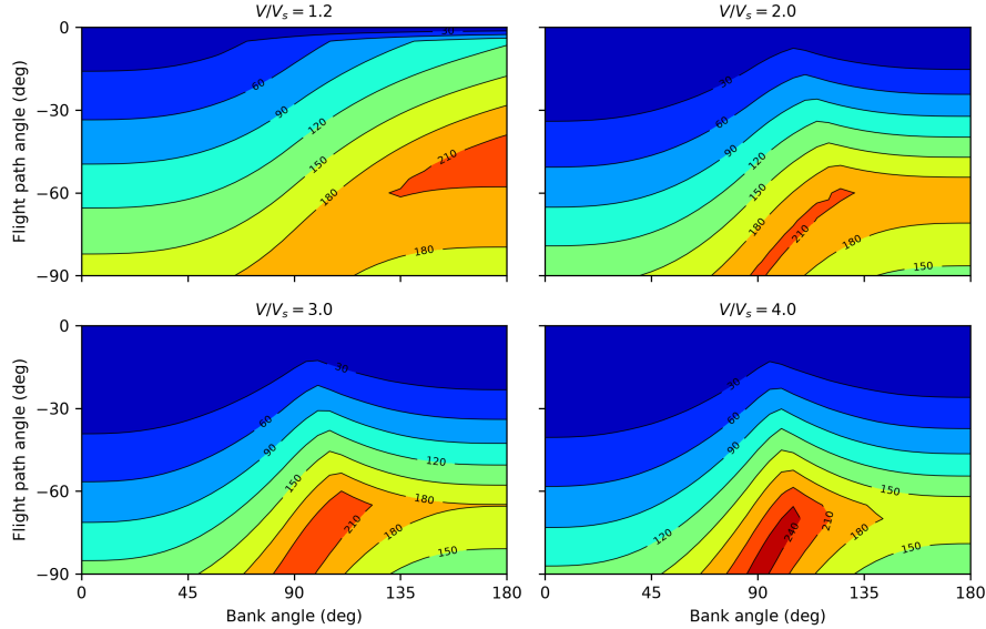
Fig. 11 Contour plots of minimal altitude loss ( \Delta h_{min} \approx -V^* ) during aircraft pullout maneuvers, evaluated on the baseline 53,280-state grid. Each subplot presents the altitude loss across the bank angle ( \mu_0 ) and flight path angle ( \gamma_0 ) envelope for a fixed initial airspeed ( V_0/V_s ). The global topology of the solution reproduces the established literature [2], validating the accuracy of the on-the-fly RK4 integration and the consistency of the barycentric interpolator.
