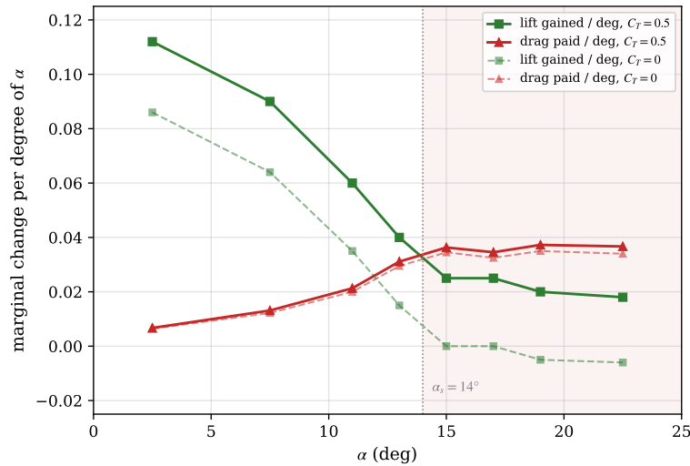
Fig. 4 The marginal trade encoded in the Riley tables: lift gained vs. drag paid per degree of angle of attack, at both propulsive conditions (finite differences at the table segment midpoints). The curves cross near \alpha_s = 14^\circ with or without power: past it, each further degree costs more drag than the lift it buys, even though the power-on lift keeps rising (Fig. 2a). The shaded region marks the unfavourable trade.
