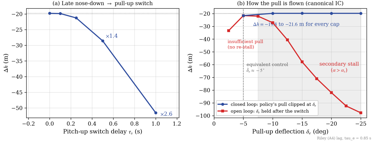
Fig. 10 Sensitivity of the recovery to pilot execution errors at the canonical IC. (a) Delaying the nose-down → pull-up switch by \tau_s , with the loss multipliers annotated. (b) The pull phase flown in its two modes, on one signed deflection scale (axis inverted so that pulling harder reads rightward): closed loop (blue), the policy with its pull commands clipped at \delta_e ; open loop (red), the same deflection held constant after the switch. Dotted line: the optimal loss; dashed vertical: the equivalent control \bar{\delta}_e \approx -5^\circ ; shaded: the held pulls that re-stall the wing ( \alpha > \alpha_s ). Note that the abscissa means a different thing for each curve: the deflection actually flown for the open loop, only a ceiling for the closed loop.
