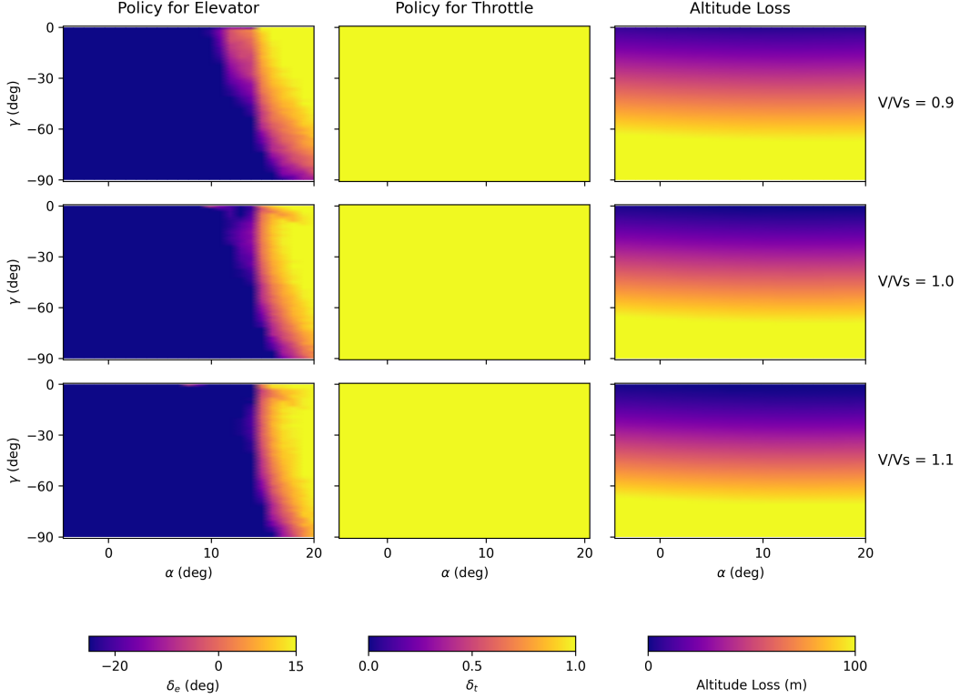
Fig. 3 Exact DP heatmaps for the 4-DOF symmetric stall recovery with the Riley (1985) propulsion-coupled aerodynamic model: optimal commanded elevator ( \delta_e^* ), throttle ( \delta_t^* ), and the value function read as minimum altitude loss, -V(\mathbf{x}) , over the evaluated flight envelope (slice q = 0 ). -V is the solver’s cost-to-absorption, not the closed-loop metric of the tables and trajectory figures, which execute the blended policy under the dive-and-return rule; the two agree in structure and differ in level by 1–3 m (see text). The elevator panels plot the raw arg max, so the narrow bands of saturated command that appear near \gamma \approx 0 should be read as the switching surface itself rather than as physical reversals: sampling the one-step Q across the full elevator range at those cells spreads it by only 0.04 m out of a 16–18 m cost-to-go (0.2%), so the extremum that wins the tie flips between adjacent rows while -V stays smooth. The blend of Sec. V.C, which is what the closed loop executes, averages across those ties.
