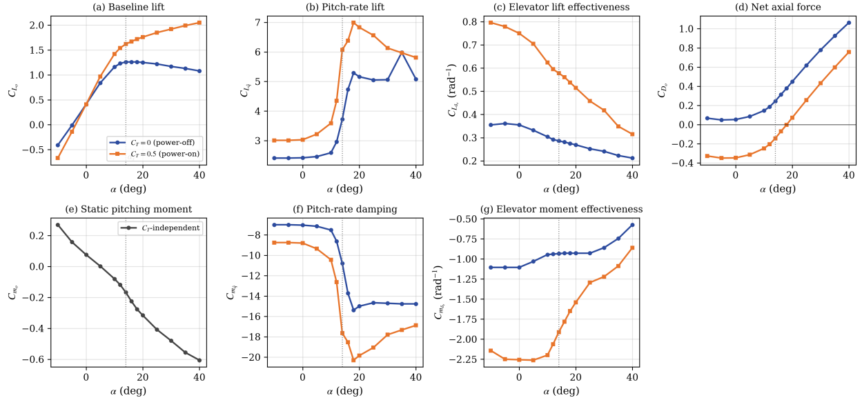
Fig. 2 The seven Riley (1985) Table III coefficients vs. angle of attack at the two tabulated propulsive conditions (one panel per table of Appendix B; C_{m_o} is C_T -independent). Three features drive the recovery physics: (a) baseline lift C_{L_o} shows the power-off flat-top stall plateau vs. monotone power-on growth from slipstream augmentation; (d) the negative power-on values of the net axial-force coefficient C_{D_o} are the embedded-thrust fingerprint of Eq. (14); (f) pitch-rate damping C_{m\dot{q}} more than doubles across the stall. The dotted line marks the stall angle \alpha_s = 14^\circ .
