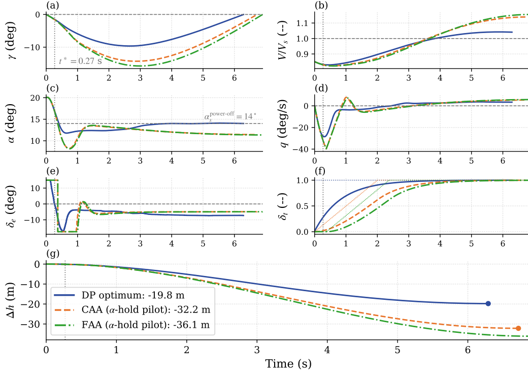
Fig. 6 Time-domain comparison at the canonical deep-stall initial condition: exact DP policy (blue, solid) vs. the scripted CAA (orange, dashed) and FAA (green, dash-dotted) procedures of Table 7. Panel (f) isolates the protocol difference, and separates what the pilot commands (dotted) from what the engine delivers (solid) through Riley’s first-order lag, \tau_e = 0.85 s: full power commanded at t = 0 (DP), a 2 s ramp from t = 0 (CAA), the same ramp from the unstall event (FAA); final losses in panel (g). The vertical dotted line marks the DP policy’s elevator-switch instant t^* = 0.27 s, the reference event for the pilot-error study of Sec. V.H. Both scripted pilots are held to the same pull authority as the optimum ( \delta_e \geq -17.50^\circ at this entry), so the figure isolates the timing of the power application rather than confounding it with how hard the pilot hauls back. The DP traces execute the policy through the barycentric action blend of Sec. V.C; the intermediate deflections and throttle settings of panels (e)–(f) are convex combinations of the discrete extremes, not commands the optimizer selected: the underlying policy is bang-bang, and holds full throttle throughout. The dashed line in panel (c) is the power-off stall boundary of the Riley tables, \alpha_s = 14^\circ ; the superscript qualifies the boundary, not the state of the aircraft, which holds full throttle throughout. Under power the lift curve continues to rise past that value, so the optimum’s excursion above the line is not a re-stall.
