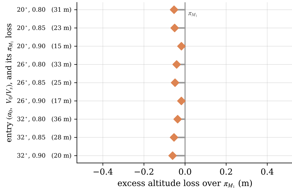
(C) m/m_0 = 1.00 , CG 10% fwd (715 kg) retrained policy loses 15 to 36 m
