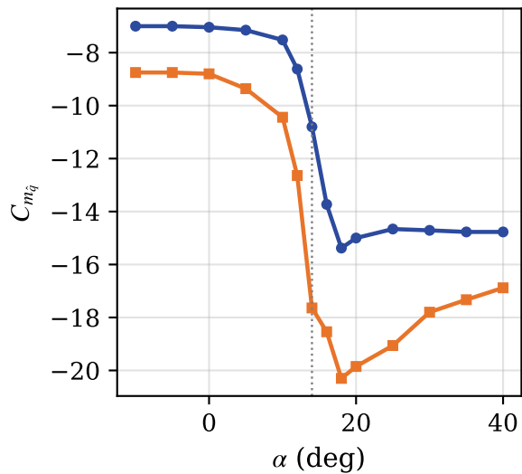
(f) Pitch-rate damping
