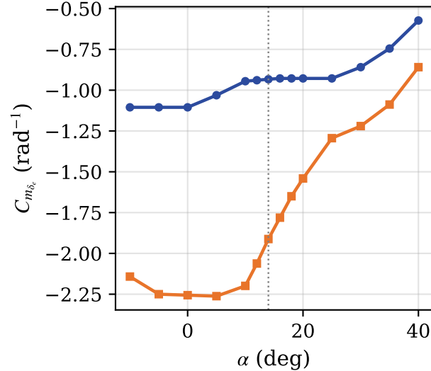
(g) Elevator moment effectiveness
