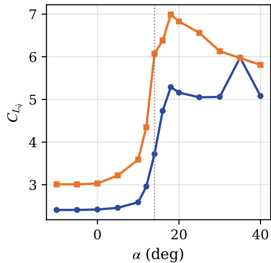
(f) Pitch-rate damping
