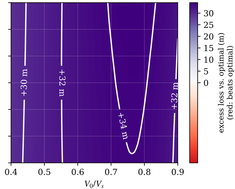
Power-delayed (Gratton: 2 s pause + 2 s ramp)
