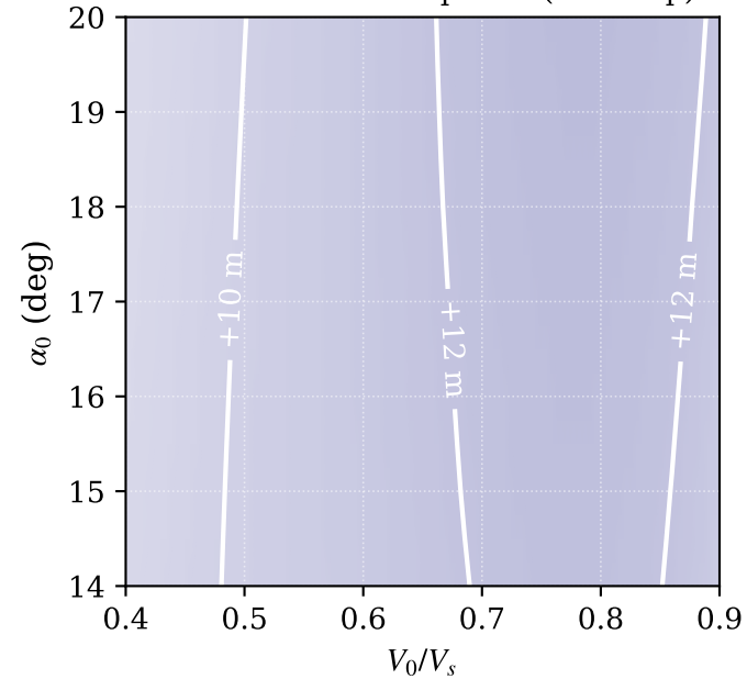
CAA: simultaneous power (2 s ramp)
