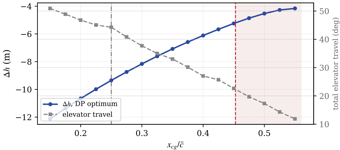
(b) The recovery the policy flies
