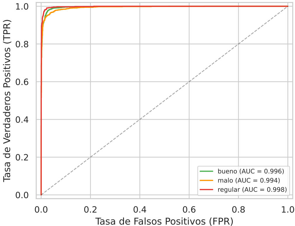
Curvas ROC — Random Forest
