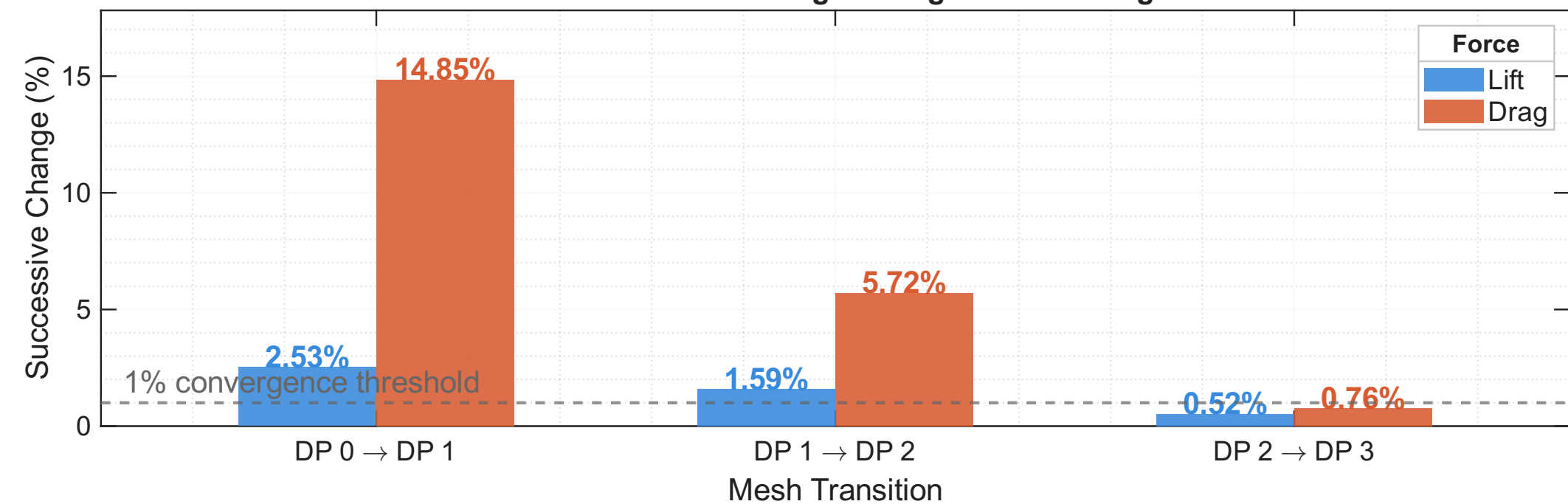
Successive Percentage Change in Lift & Drag
