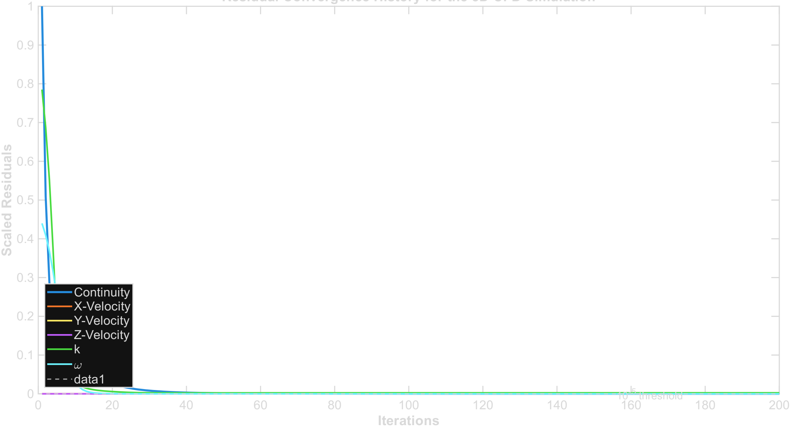
Residual Convergence History for the 3D CFD Simulation
