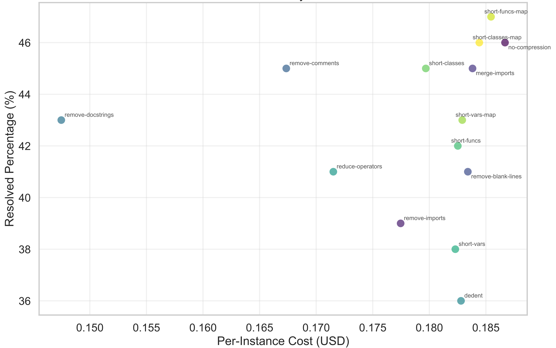
Performance vs Cost by Transformation
