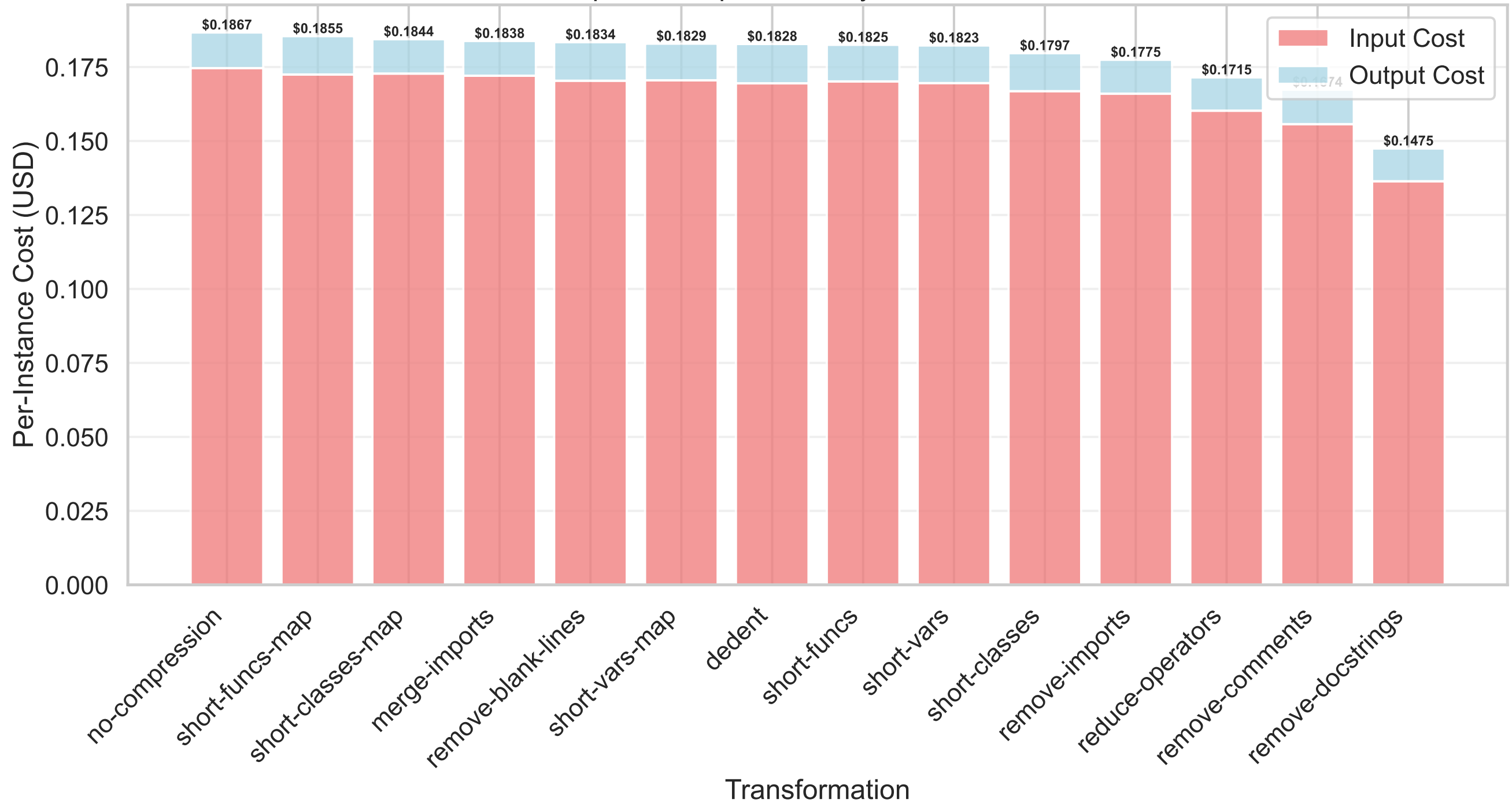
Input vs Output Costs by Transformation
