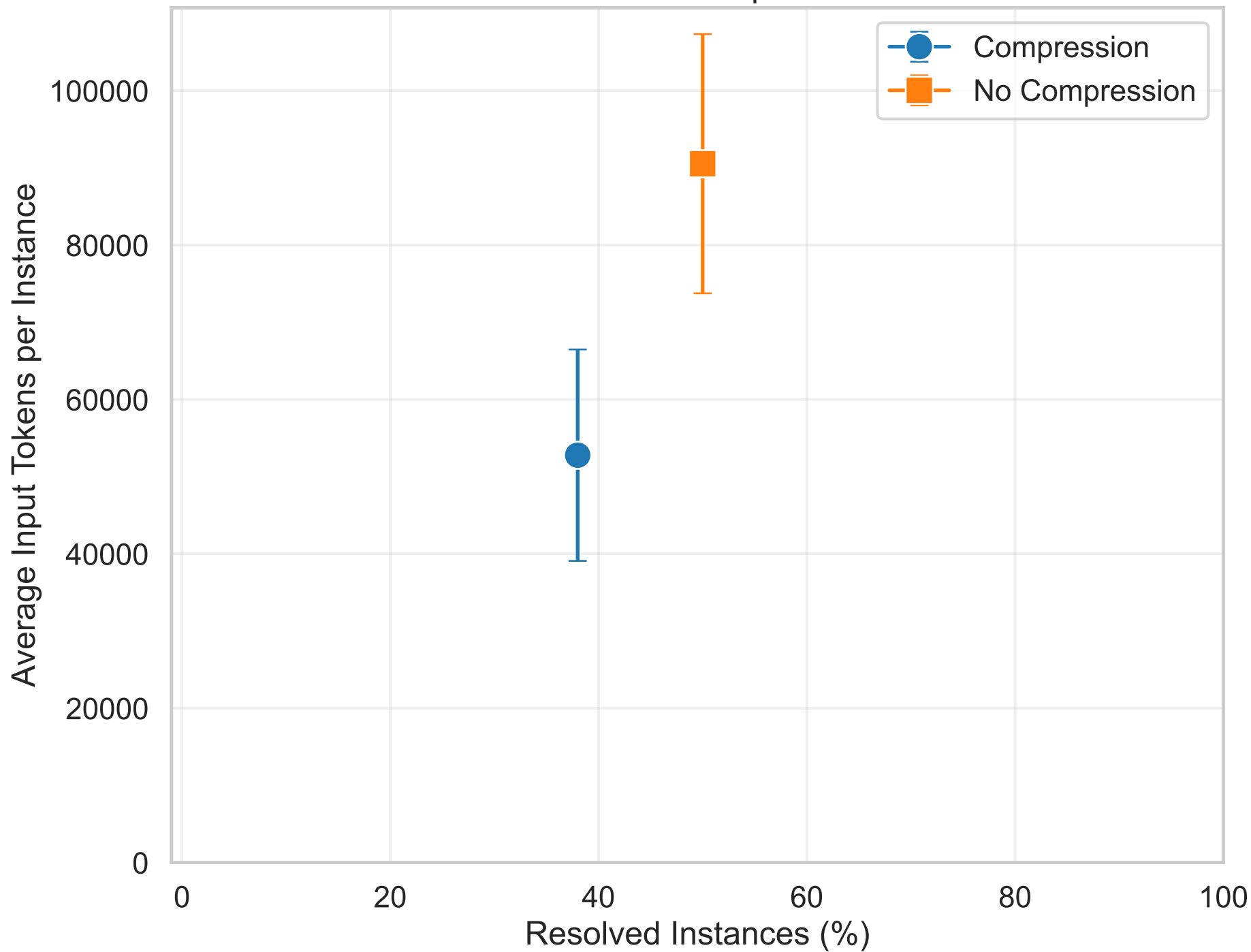
Performance vs Input Tokens
