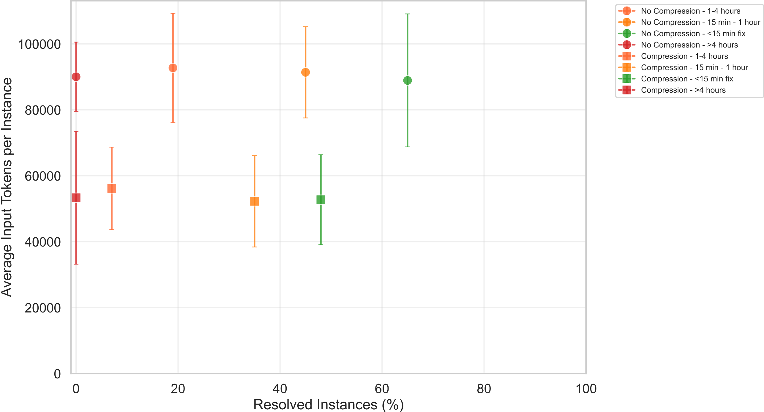
Performance vs Input Tokens by Difficulty Level
