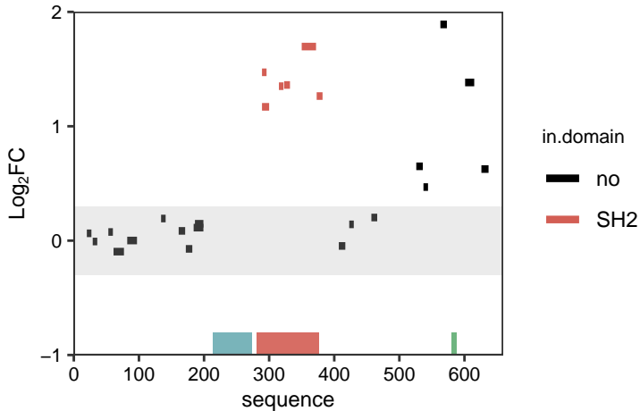
BTK, Dasatinib_crude
